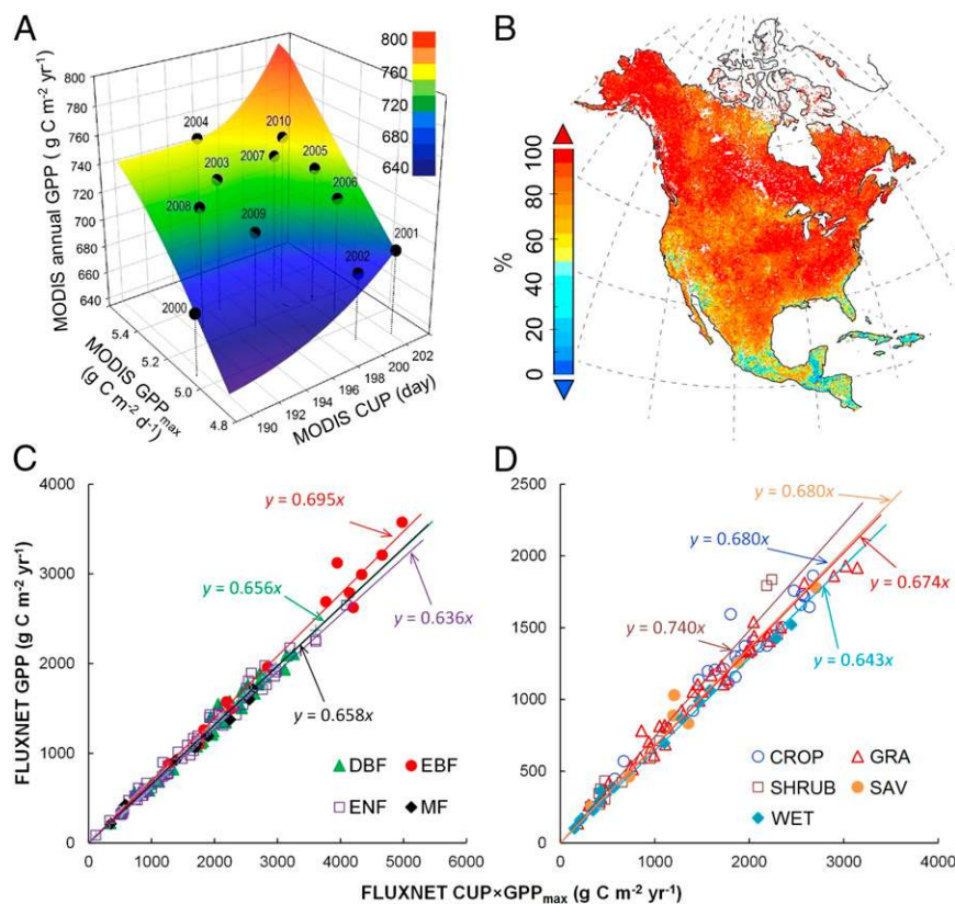
Fig. 1. Joint control of the temporal variability of satellite-derived annual GPP and the spatial variability of FLUXNET annual GPP by CUP and GPP max . (A) The temporal variability of GPP in North America from 2000 to 2010 can be better understood by splitting annual GPP into GPP max and CUP. The flat color interpolated surface reflects a good relationship between annual GPP and GPP max × CUP ( R^2 = 0.95 , P < 0.001 ). Vertical lines were added to improve readability. (B) Contribution of GPP max × CUP to GPP temporal variability over 2000–2010. The contribution in each grid cell was derived from the R^2 in the linear regression analysis between GPP and GPP max × CUP. C and D show relationships between GPP and GPP max × CUP across FLUXNET sites in forest and nonforest biomes, respectively. Each data point in C and D represents one flux site with average data over different years. CROP, cropland; DBF, deciduous broadleaf forest; EBF, evergreen broadleaf forest; ENF, evergreen needleleaf forest; GRA, grassland; MF, mixed forest; SAV, savanna; SHRUB, shrubland; WET, wetland.
