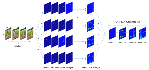
Figure 1: Dynamic pose image (DPI) for action description from a video. All generated images are colored to facilitate observation.
