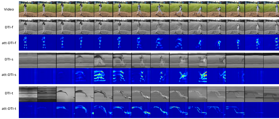
Figure 2: Comparison between DTIs and att-DTIs. Three att-DTIs are colored to facilitate observation.
