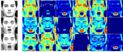
Figure 6. Feature maps corresponding to Figure 5. The gray images on the left side form the image sequence used as input, and the images on the right side are the feature maps corresponding to each filter in Figure 5. Blue and red represent the low and high response values. The emotion label for the input image sequence was surprise. We observed that our network responded to moving parts for expressing emotion.
