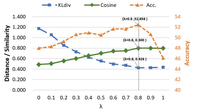
Figure 3: Effect of \lambda on the Emotion6 dataset, which indicates the weight of the distribution term in the optimization objective function. Note that \lambda = 0 represents that only softmax loss for classification is employed.
