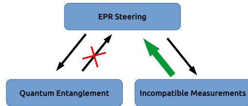
Figure 1. The observation of EPR steering, a form of quantum nonlocality, implies the presence of both entanglement and incompatible measurements. Whether the converse links hold is an interesting question. Here we make progress in this direction by showing that any set of incompatible measurements can be used to demonstrate EPR steering (green arrow).
