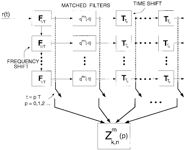
Fig. 5. Implementation of sampled STFT using a bank of identical matched filters determined by the signaling waveforms. Z_{k,n}^m(p) denotes the sufficient statistics for the p th symbol; that is, Z_{k,n}^m(p) = \langle r_p, u_{k,n}^m \rangle , where r_p(t) = r(t + pT) . Note that each matched filter branch corresponds to a conventional RAKE receiver.
