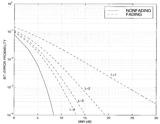
Fig. 2. BEP versus SNR for coherent antipodal signaling over AWGN (solid) and Rayleigh fading (dashed) channels. The dashed curves represent different levels ( L = 1, 2, 3, 4 ) of diversity. Monotonic improvement as a function of L is evident.
