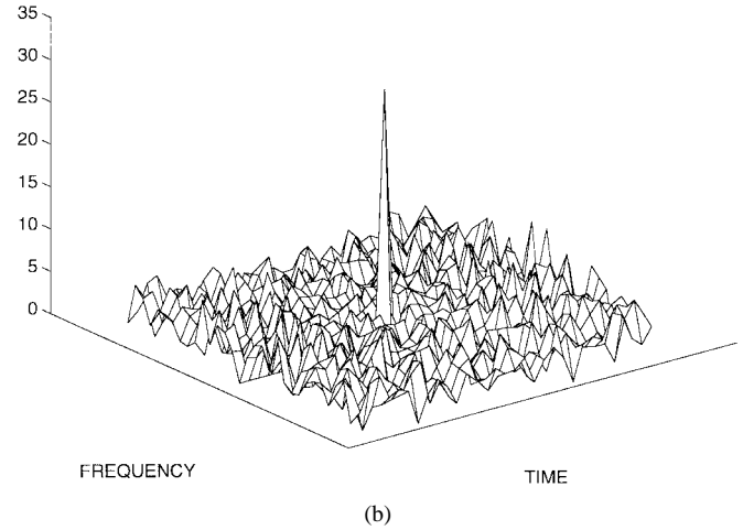
Fig. 3. (a) Sampling of the time-frequency plane to create multipath-Doppler diversity channels. (b) Sampled time-frequency correlation function of a spread-spectrum signaling waveform (length-31 M-sequence).
