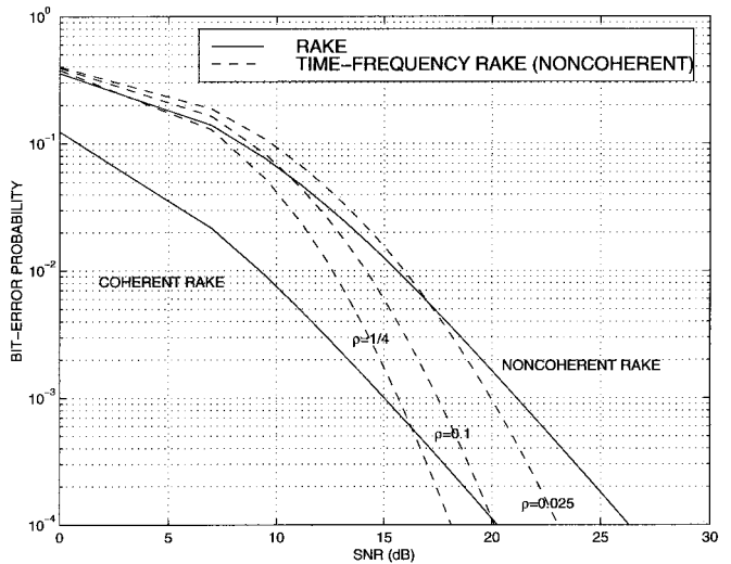
Fig. 8. Joint multipath-Doppler diversity gains as a function of \rho for noncoherent equal-gain combining (no channel knowledge) and N = 2 multipath components. The coherent RAKE receiver (antipodal signaling) signifies the optimal performance of existing systems under slow fading. The noncoherent RAKE receiver (orthogonal signaling) typifies the degraded performance of existing systems under fast fading. Note that the noncoherent time-frequency RAKE receiver provides a lower bound on the performance of proposed systems.
