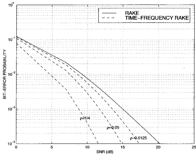
Fig. 7. Joint multipath-Doppler diversity gains as a function of \rho for coherent antipodal signaling (perfect channel knowledge) and N = 2 multipath components. The performance of the RAKE receiver is under (ideal) slow fading ( TB_d = 0 , \rho = 0 ).
