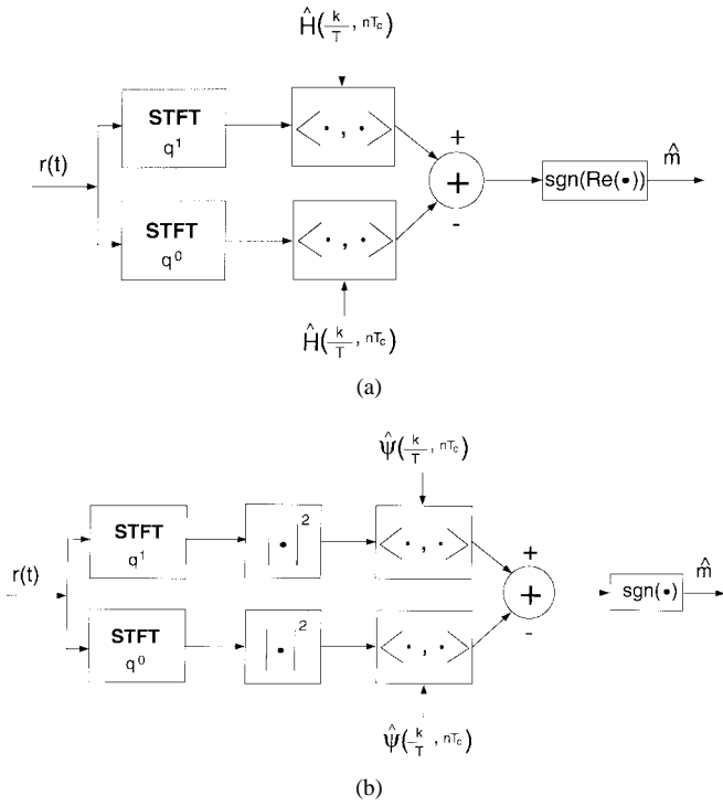
Fig. 4. STFT-based detector structures (time-frequency RAKE receivers) for exploiting joint multipath-Doppler diversity: (a) coherent processing and (b) noncoherent processing.
