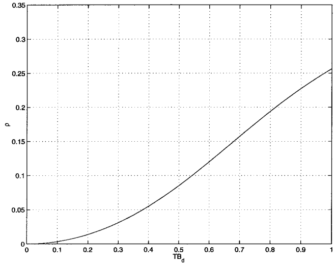
Fig. 6. The variation in \rho as a function of the product TB_d .
