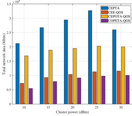
Fig. 9: Total network data for CEE-QoS and CEPTA, CEPOTA-QoS, COPETA-QoS.
