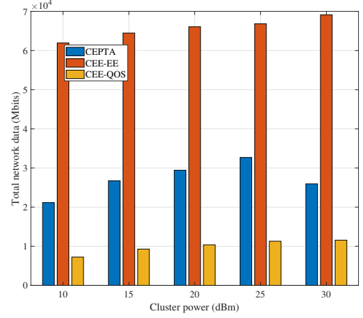
Fig. 7: Total network data for CEE-EE, CEE-QoS and CEPTA.
