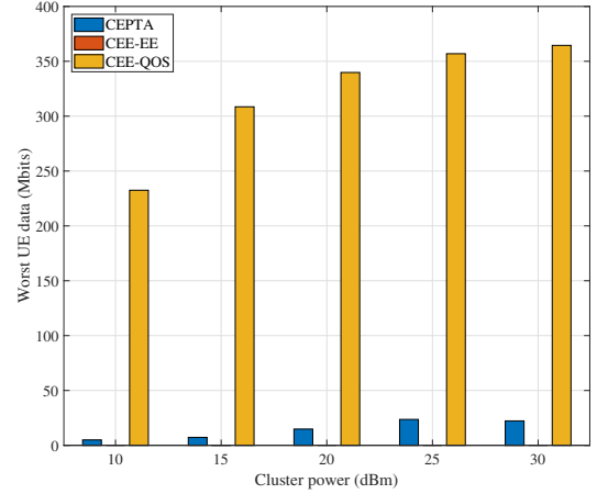
Fig. 8: Worst UE data for CEE-EE, CEE-QoS and CEPTA.
