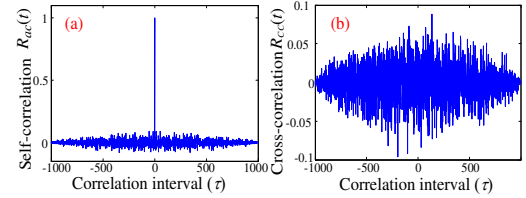
Fig. 6. The statistical correlation curves of chaotic sequence. (a) Self-correlation curves of chaotic sequence a_j ; (b) Correlation curves of chaotic sequences a_j and a_h .
