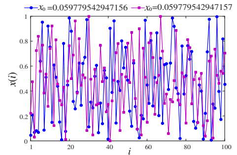
Fig. 3. The sensibility of 2D Logistic map to change of the initial value x_0 .
