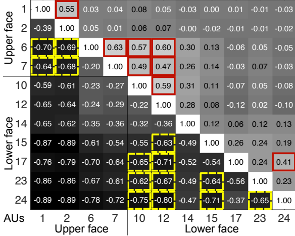
Figure 4. The relation matrix studies on more than 350,000 valid frames with AU labels. Red solid and dashed yellow rectangles, respectively, indicate the relations of positive correlations and negative competitions studied in this work.
