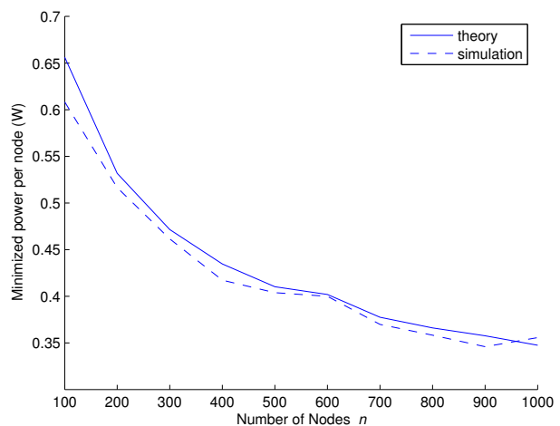
Fig. 7. Minimized power per node, computed using the steady-state probabilities from Figure 5. The transmission/sensing radius is kept constant at r = 0.2 and the sensing event probability at P_{SE} = 0.1 .
