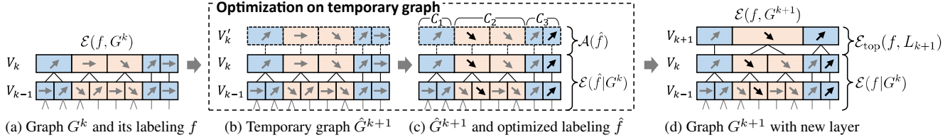
Figure 3. Bottom-up Graph Construction (one step) . Each rectangular cell in the illustration represents a node i \in V_l and a set of contiguous cells represents a graph layer V_l . The arrows and colors denote flow and alpha labels f_i (red: foreground, blue: background). (a) Graph G^k and its labeling f . (b) By duplicating the top layer V_k of G^k , we create a temporary graph \hat{G}^{k+1} as an approximation of G^{k+1} . (c) We optimize the labeling \hat{f} on \hat{G}^{k+1} . The number of unique labels in V'_k is reduced by label costs [15] to induce region merging. (d) V'_k is converted into a new layer V_{k+1} , by merging nodes of V'_k assigned the same label that form connected components in G^{k+1} .
