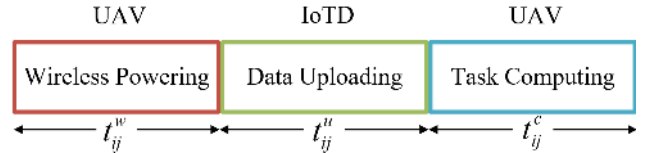
Fig. 2. Three stages of one service flow
