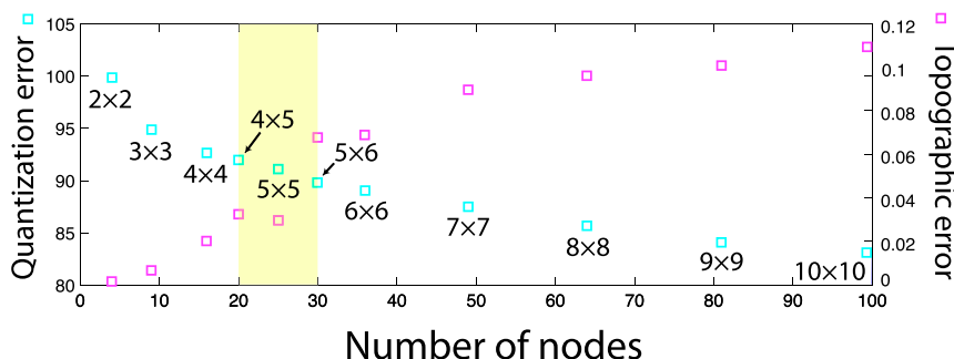
FIG. 2. Elbow plot used to evaluate the optimal number of nodes. Quantization error (m) decreases with an increasing number of nodes while topographic error increases with an increasing number of nodes. The optimal number chosen is 25 nodes, highlighted in the region shaded with yellow. Note that the nonsquare map orientations are wider than they are tall.
