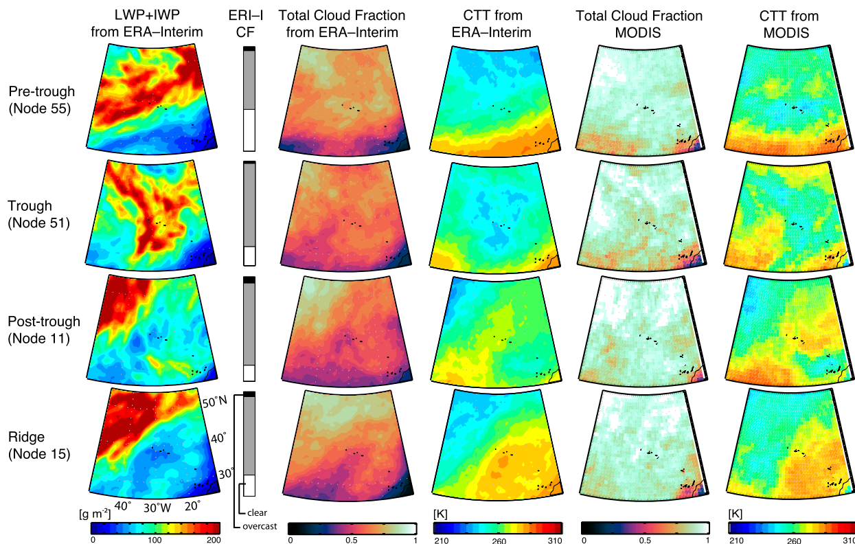
FIG. 9. As in Fig. 7, but for January.
