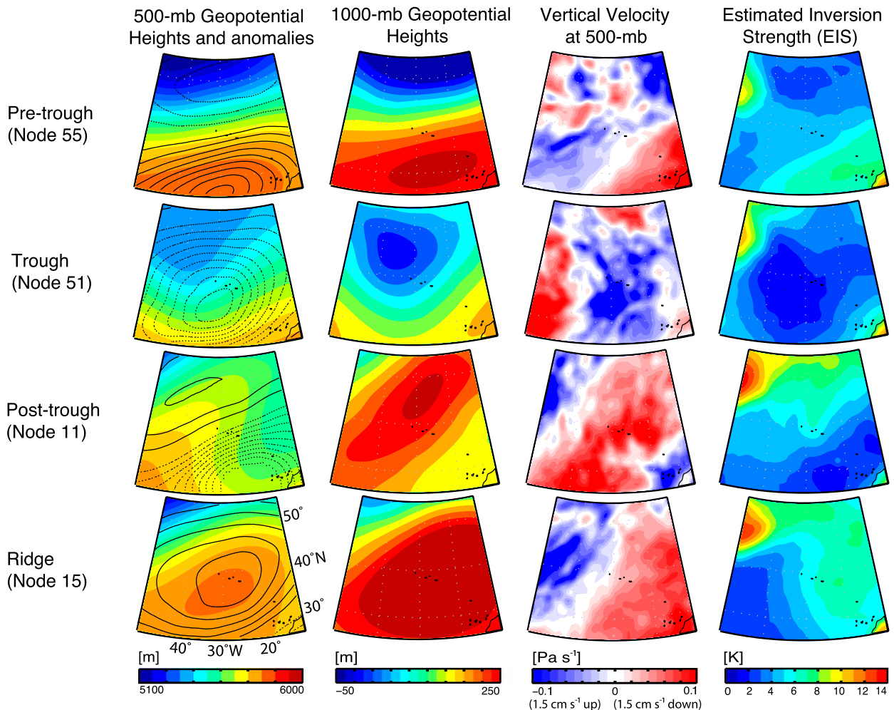
FIG. 8. As in Fig. 6, but for January. The 5 \times 5 node map for January from which these specific nodes are drawn (corresponding to Fig. 3 for the June nodes) is shown in supplemental Fig. S1.
