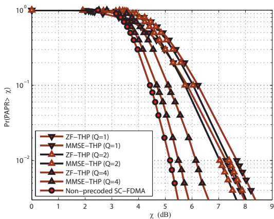
Fig. 4. PAPR Characteristics of the precoded SC-FDMA waveform.
