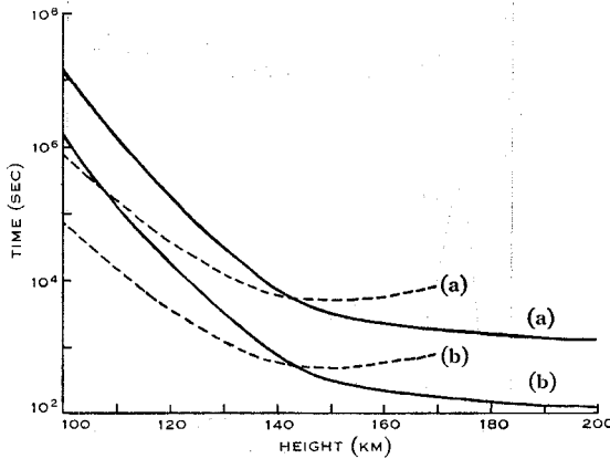
Fig. 1.—Full line, graph of \alpha^{-1} ( =\rho/\sigma_1H^2 ); dashed line, graph of \beta^{-1} ( =\rho/\sigma_3H^2 ); curves (a) refer to Chapman's h -model atmosphere (see Fig. 2) and curves (b) to a disturbed atmosphere with electron density 10 times the former.
