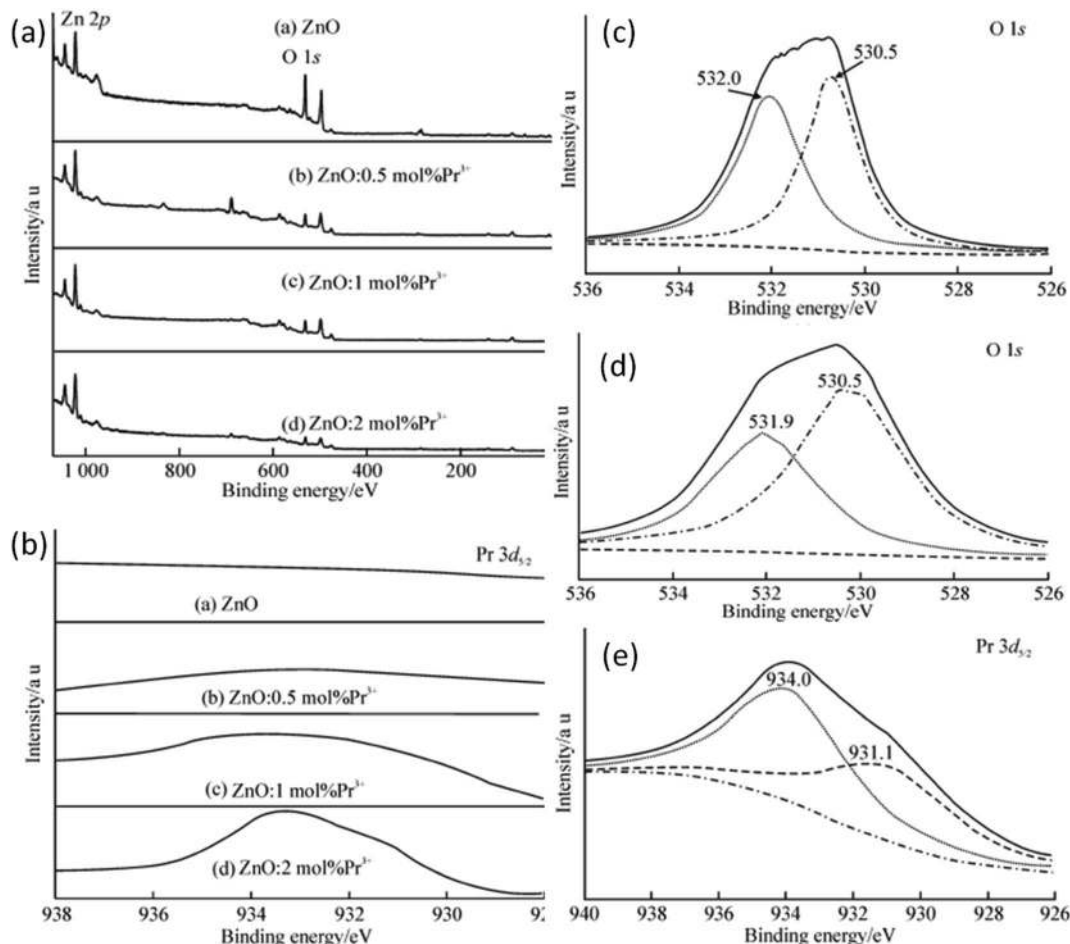
Fig. 14 (a) XPS spectra of \text{Pr}^{3+} -doped ZnO QDs, (b) binding energy scan of \text{Pr}^{3+} -doped ZnO QDs for \text{Pr } 3d_{5/2} , (c and d) fitting spectra of O 1s from undoped and 2 mol% \text{Pr}^{3+} -doped ZnO QDs, respectively and (e) XPS spectrum of \text{Pr } 3d_{5/2} from 2 mol% \text{Pr}^{3+} -doped ZnO QDs. 38 Adapted with permission from ref. 38. Copyright (2014) Springer.
