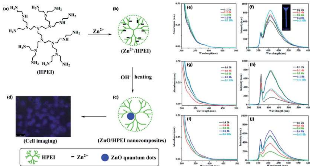
Fig. 23 (a–d) Illustration of the ZnO/HPEI nanocomposite and the fluorescent cell imaging, UV-Vis and PL spectra of ZnO QDs at [Zn 2+ /OH - ] molar ratio of (e and f) 1 : 2, (g and h) 1 : 1, and (i and j) 1 : 4. 124 Adapted with permission from ref. 124. Copyright (2020) Elsevier.
