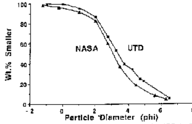
Figure 3. Particle size distribution curves for JSC-1. Particle diameters in phi units ( \phi = -(\ln d) / (\ln 2) , d = diameter in mm).
