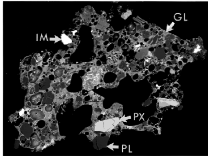
Figure 5. Lunar mare soil grain (78221,8) in polished section. Phases include glass (GL), plagioclase (PL), pyroxene (PX), and ilmenite (IM). SEM back-scattered electron image. Frame width = 660 \mu\text{m} .
