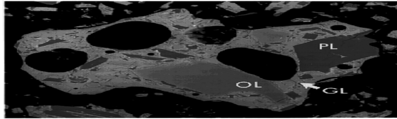
Figure 1. JSC-1 grains in polished section. Phases include glass (GL), plagioclase (PL) and olivine (OL). SEM back-scattered electron image. Frame width = 520 \mu\text{m} .
