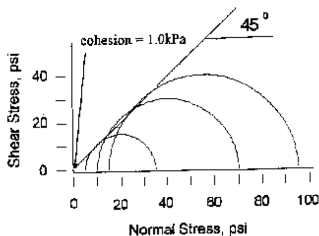
Figure 4. Mohr stress circles used to determine angle of internal friction ( 45^\circ ) and cohesion (1.0 kPa) for JSC-1.
