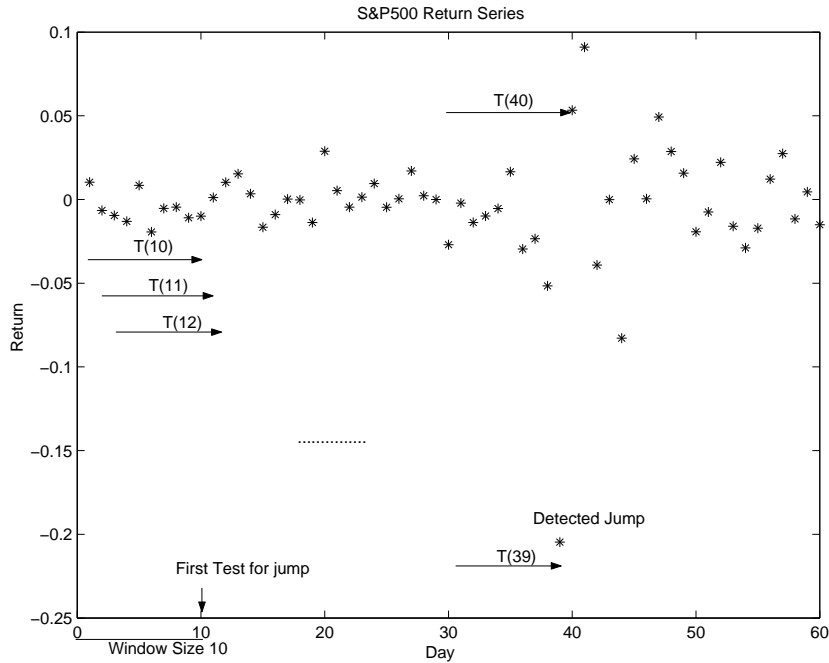
Figure 1: Intuition of Jump Detection Test
