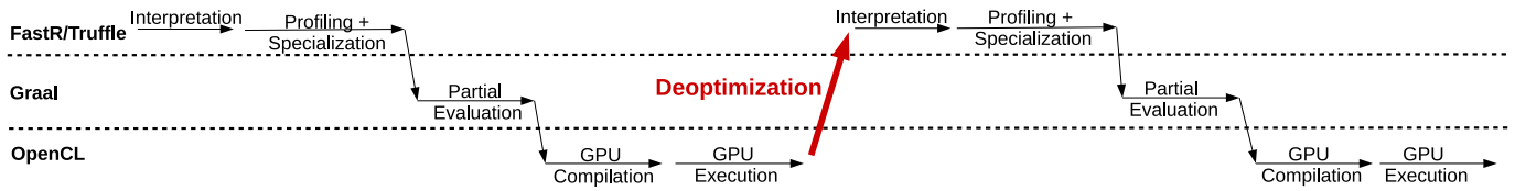
Figure 5: Execution of an R program which gets specialized, compiled to the GPU, before a deoptimization is performed, the program is re-profiled and generalized, compiled to the GPU again, and, finally, successfully executed on the GPU.
