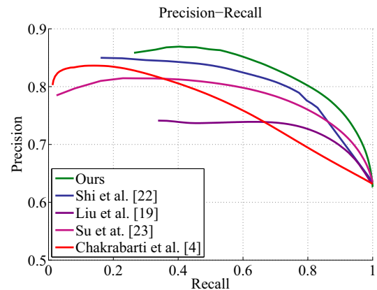
Figure 9. Precision-recall comparison on the blur dataset [22].
