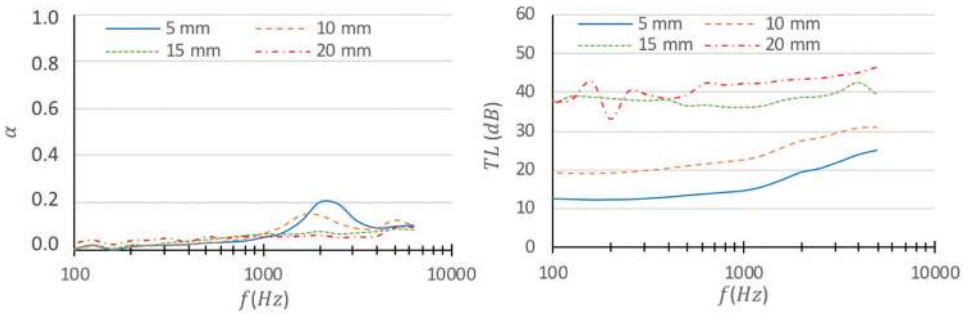
Figure 2. The SACs (left) and TLs (right) of the jute composite samples with different thicknesses (density: 997.6 \text{ kg/m}^3 , fiber/epoxy ratio: 0.6).
