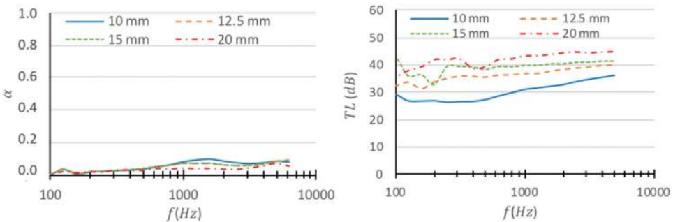
Figure 3. The SACs (left) and TLs (right) of the luffa composite samples with different thicknesses (density: 829.9 \text{ kg/m}^3 , fiber/epoxy ratio: 0.45).
