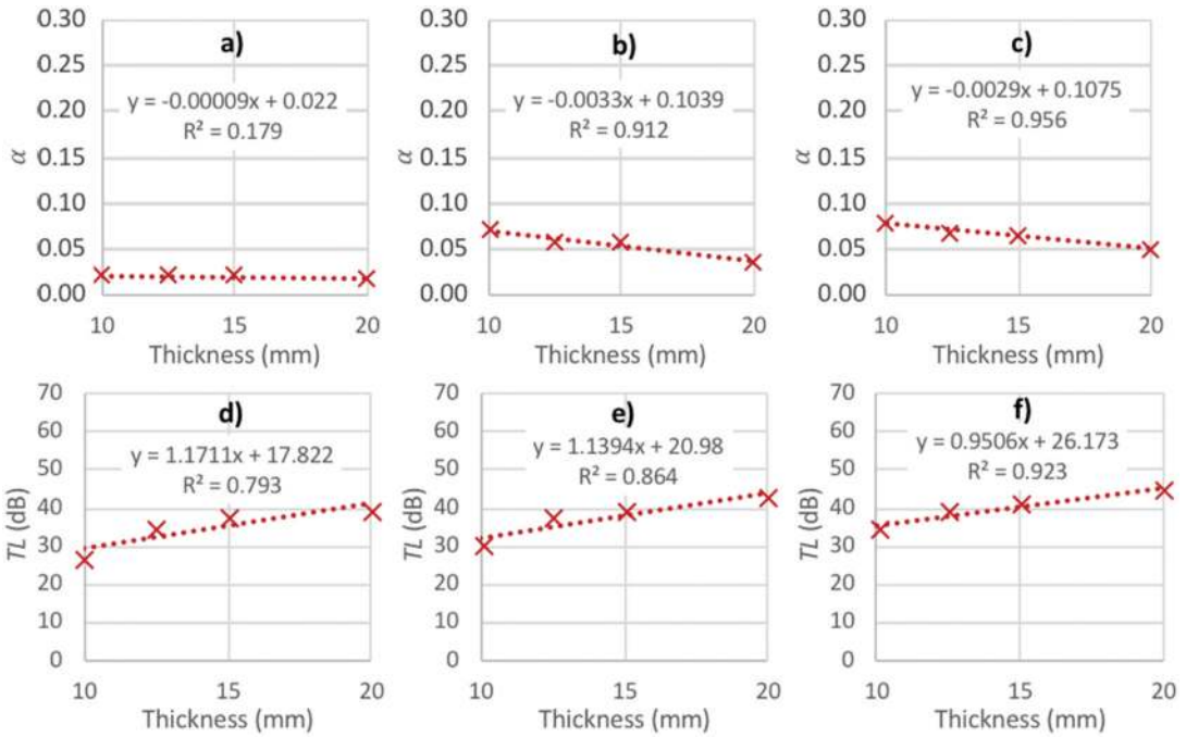
Figure 7. The average SACs and TLs of the luffa composite samples with different thicknesses for low (a and d), medium (b and e) and high (c and f) frequency ranges (density = 829.9, luffa fiber/epoxy ratio = 0.45).
