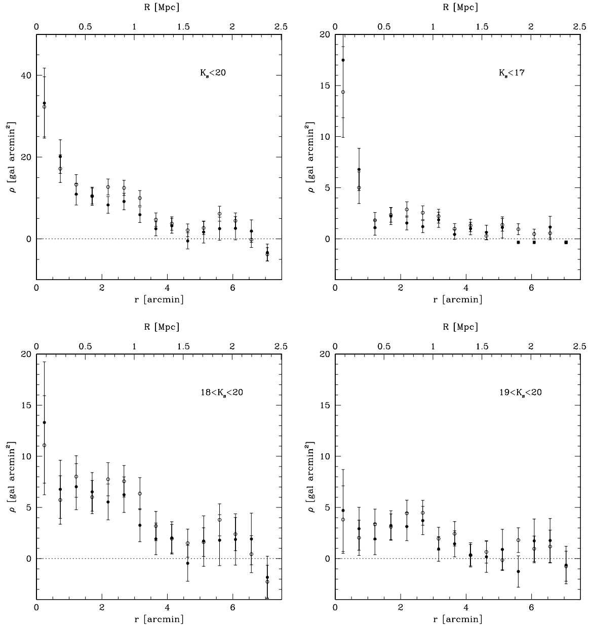
Fig. 2. Background subtracted radial profiles of the AC118 cluster. Galaxies having K_s < 20 , K_s < 17 , 18 < K_s < 20 and 19 < K_s < 20 mag are selected for the computation of the radial profiles in the top-left, top-right, bottom-left and bottom-right panels, respectively. Open dots show the profile computed over all the observed field, while closed points show the profile computed excluding the southeast 1 arcmin and the NW quadrant. Note the steepness of the radial profile of bright galaxies (upper-right panel) and the flatness of the radial distribution of faint galaxies (lower-left panel). The density of background galaxies measured in the HDF-S is 7.8, 0.3, 6.3, 4.2 gal arcmin ^{-2} for K_s < 20 , K_s < 17 , 18 < K_s < 20 and 19 < K_s < 20 mag respectively, when adopting our 3 arcsec aperture magnitude, and has been already subtracted.
