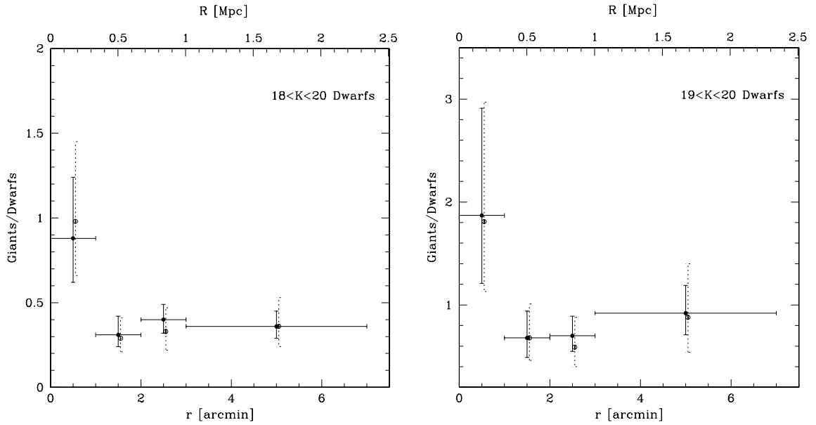
Fig. 4. Giant ( K_s < 17 ) to dwarf ( 18 < K_s < 20 in the left panel, 19 < K_s < 20 in the right panel) ratio as a function of the clustercentric distance, including and excluding the NW quadrant and the southeast 1 arcmin (open and solid points, respectively). Error bars in the abscissa show the bin width. For display purposes error bars in the abscissa are drawn once and points are slightly displaced in x .
