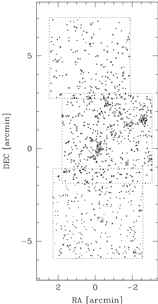
Fig. 1. Detected galaxies (ellipses), brighter than K_s = 20 mag. The area of ellipses is twice the galaxy isophotal area computed at 1.5\sigma above the background ( 20.8\text{--}21.8 mag arcsec ^{-2} ). North is up and East is to the left. The origin is at (\alpha, \delta) = (00\ 14\ 20, -30\ 24\ 00) (J2000).
