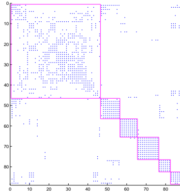
Figure 3. The connectivity matrix for lymphoma. The 6 classes are ordered as C_1, C_4, C_7, C_9, C_6, C_5 .
