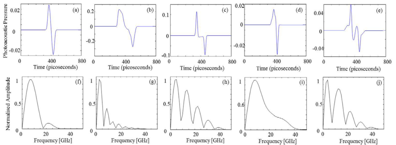
Figure 2: Photoacoustic signal and frequency spectrum of the PA signal generated from the nano particles. (a-e) photoacoustic signal generated from nanosphere, nanocylinder, nanocube, nanotriangle, and nanostar. (f-j) Frequency spectrum of the photoacoustic signal generated from nanosphere, nanocylinder, nanocube, nanotriangle, and nanostar.
