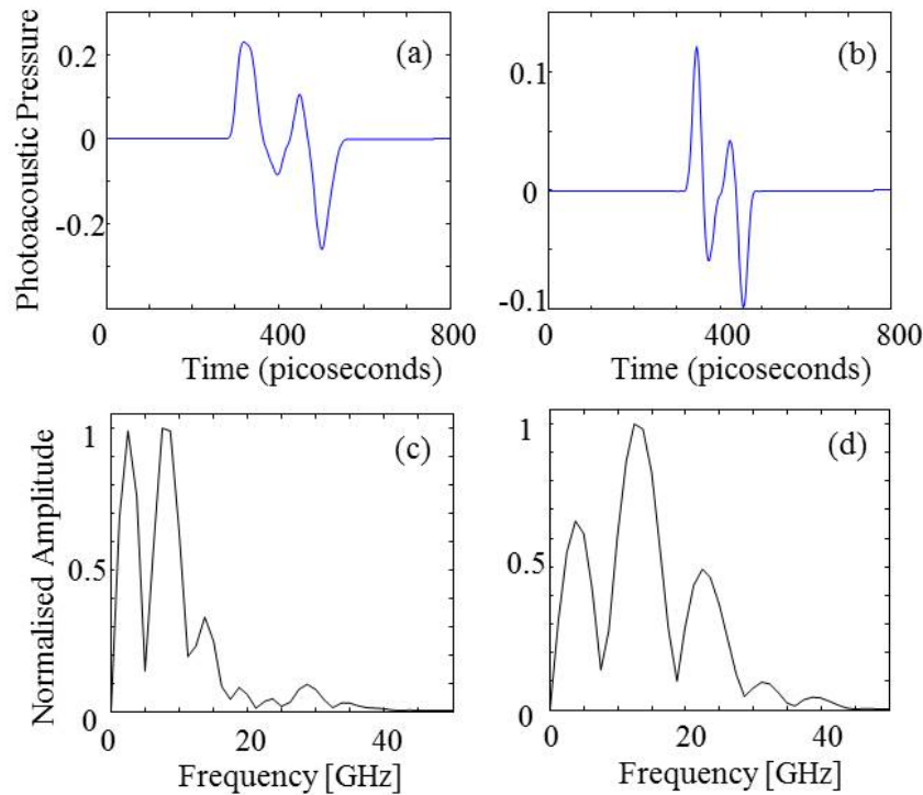
Figure 3: Photoacoustic signal and frequency spectrum of the PA signal generated from the nano particles. (a-b) photoacoustic signal generated from hollow cylinder, and hollow cube. (c-d) Frequency spectrum of the photoacoustic signal generated from hollow cylinder, and hollow cube.
