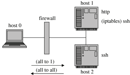
Fig. 1. An Example Network
