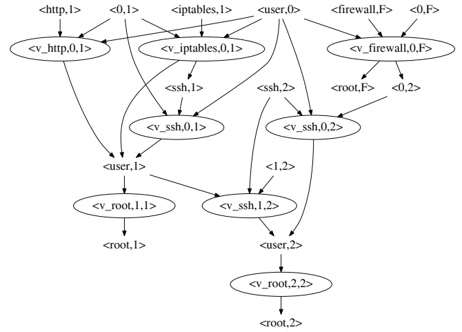
Fig. 3. An Example of Zero Day Attack Graph
