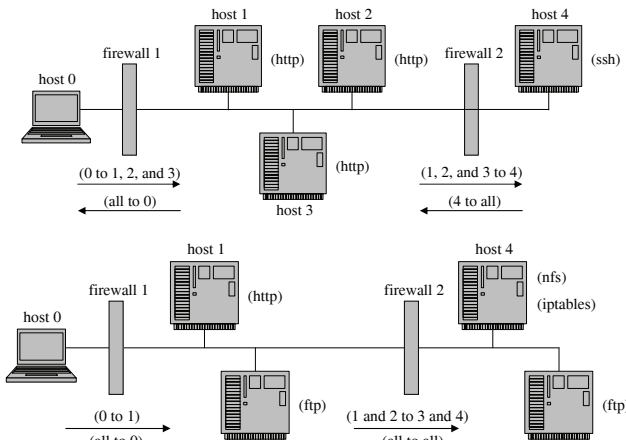
Fig. 7. Case Study: Security by Diversity
