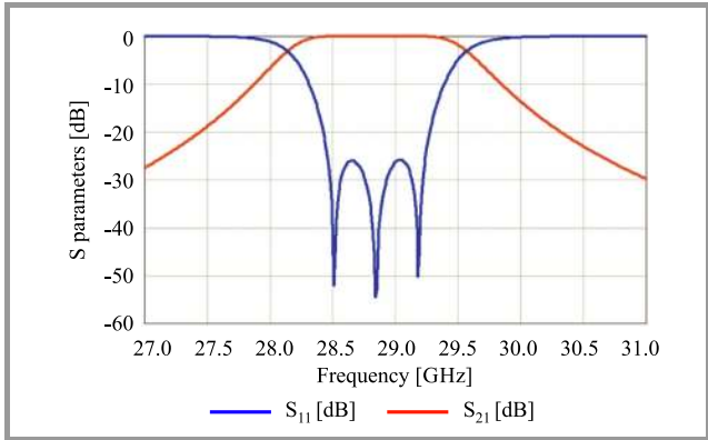
Fig. 5. Ideal response curve of the third order SIW to a band-pass filter based on the CM technique.
