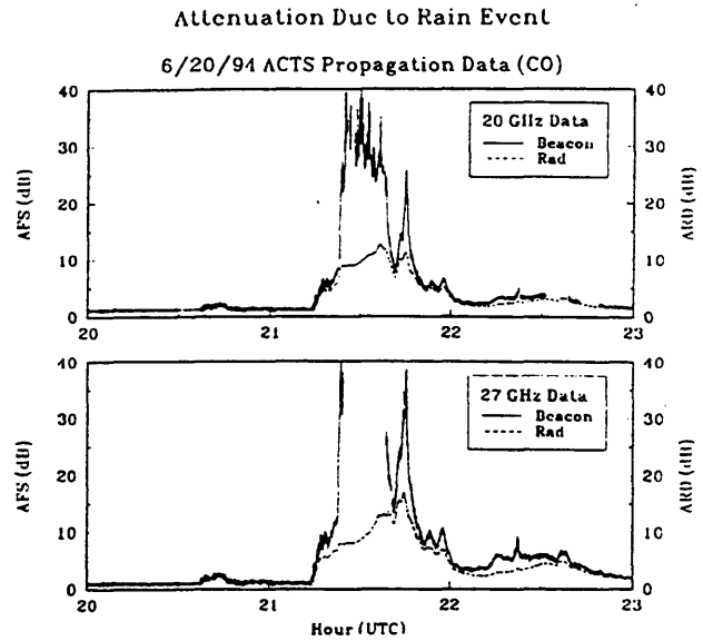
Figure 5: June 20, 1994 rain event, measured by the CSU-APT.
