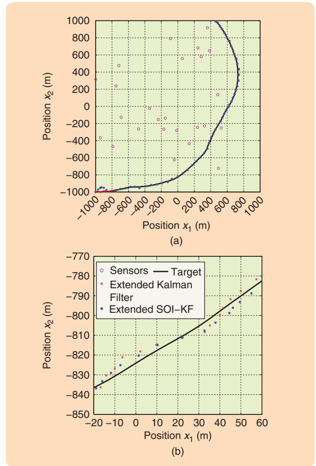
FIGURE 4 Target-tracking with the extended sign of innovations Kalman filter (SOI-KF). The entire trajectory is shown in (a), while a detail is shown in (b). The target trajectory is displayed along with extended Kalman filter estimates computed using the nonquantized amplitude observations y(n) and extended SOI-KF estimates computed using the sign of innovations messages m(n) . The extended Kalman filter and extended SOI-KF estimates are indistinguishable. The target moves according to the zero-acceleration model in (11), (12). Randomly deployed sensors provide distance-only observations of the form y_k(n) = \alpha \log \|\mathbf{p}(n) - \mathbf{p}^k\| + v(n) , where \mathbf{p}(n) is the target's position, \mathbf{p}^k is the position of the k th sensor, and v(n) is white Gaussian noise with variance \sigma_v . The scheduling algorithm works in cycles. At the beginning of each cycle, the sensor closest to the predicted estimate of the target's position \hat{\mathbf{p}}(n|\mathbf{m}_{0:n-1}) is scheduled followed by the second closest and so on, until the T th closest sensor is scheduled, completing the cycle. For this example, the parameters are T = 4 slots, T_s = 1 s, and K = 100 sensors deployed in a 2-km-by-2-km square with \alpha = 3.4 , \sigma_u = 0.2 m/s 2 , and \sigma_v = 1 .
