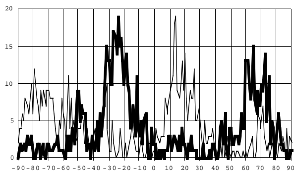
figure 6 : Angle-histograms of the two positions
