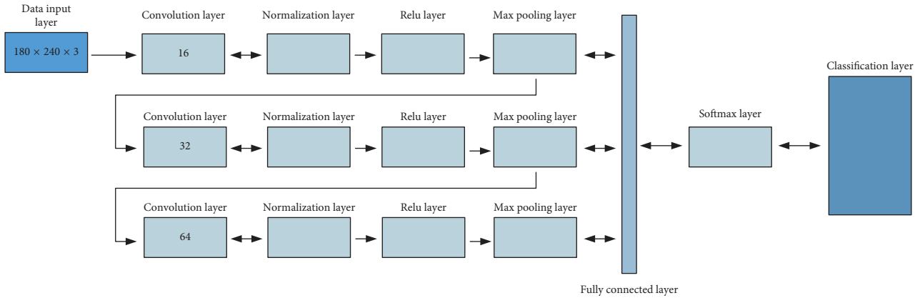
FIGURE 6: CNN-designed algorithm.
