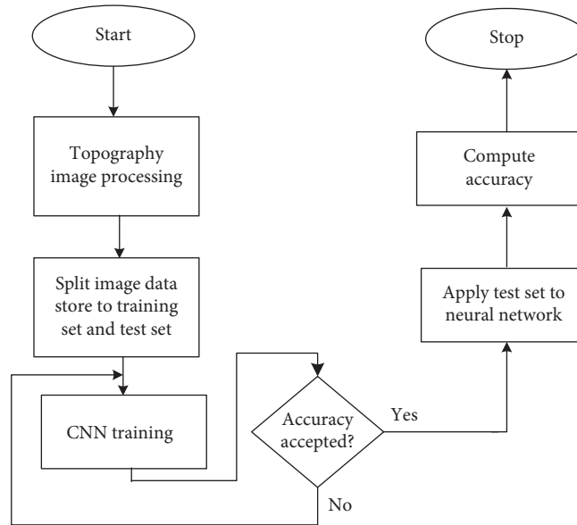
FIGURE 4: CNN-proposed algorithm.
