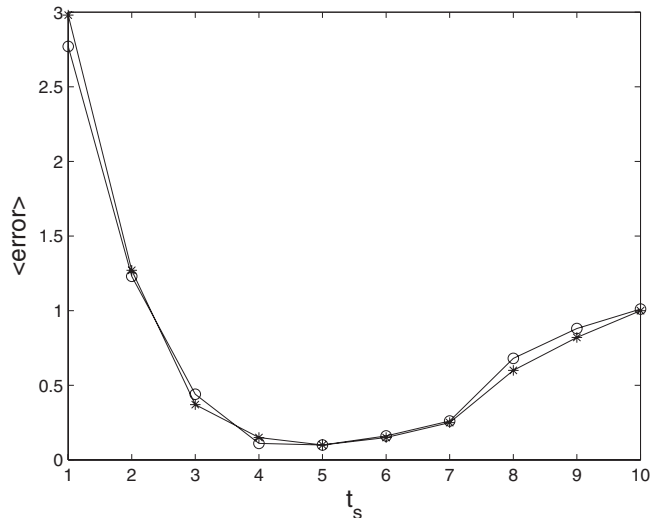
FIG. 8. Concerning the genetic regulatory network, the mean number of errors (over 100 realization of the system of length N = 2000 ) obtained using the linear IP kernel ( p=1 , empty circles) and Gaussian kernel (stars), is plotted versus the sampling time t_s . In the Gaussian case, \sigma=50 is used. The level of discretization is n_c=3 and m=2 .
