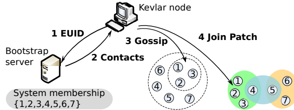
Fig. 4. Patch assignment. Upon initialization, a KEVLAR node tests its local environment to produce an EUID; (1) sends this EUID to a bootstrap server; (2) receives a contact list in return; (3) uses this list to identify other nearby members and patches via gossip; (4) applies these EUID metrics to dynamically select patches to join.
