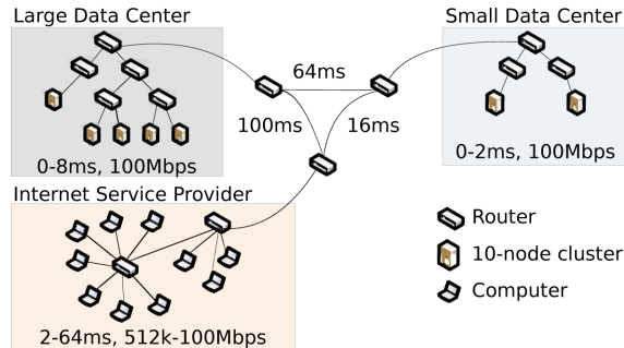
Fig. 6. Network topology. Experimental network topology, as emulated on DETERlab, with data centers and an Internet service provider: node numbers, latencies, and data rates as indicated, with IP multicast internally enabled in data centers.
