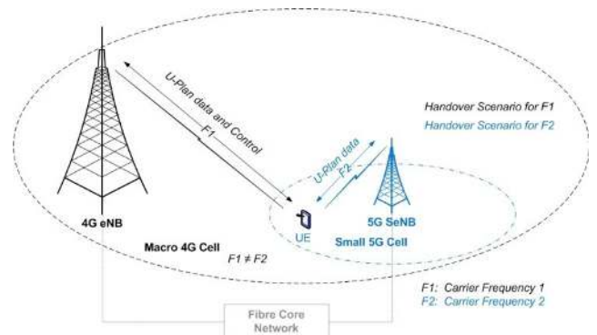
FIGURE 4. Dual Connectivity with handover scenarios in future communication networks.
