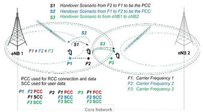
FIGURE 3. Dual Connectivity with handover scenarios in future communication networks.
