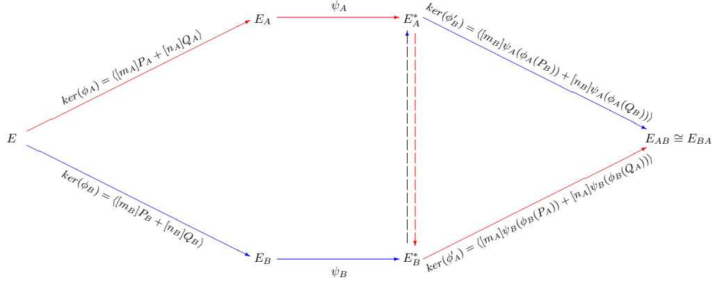
Fig. 1. Key exchange protocol with compression
