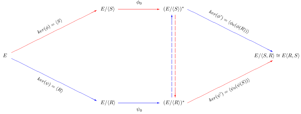
Fig. 2. Zero-knowledge proof of identity with compression
