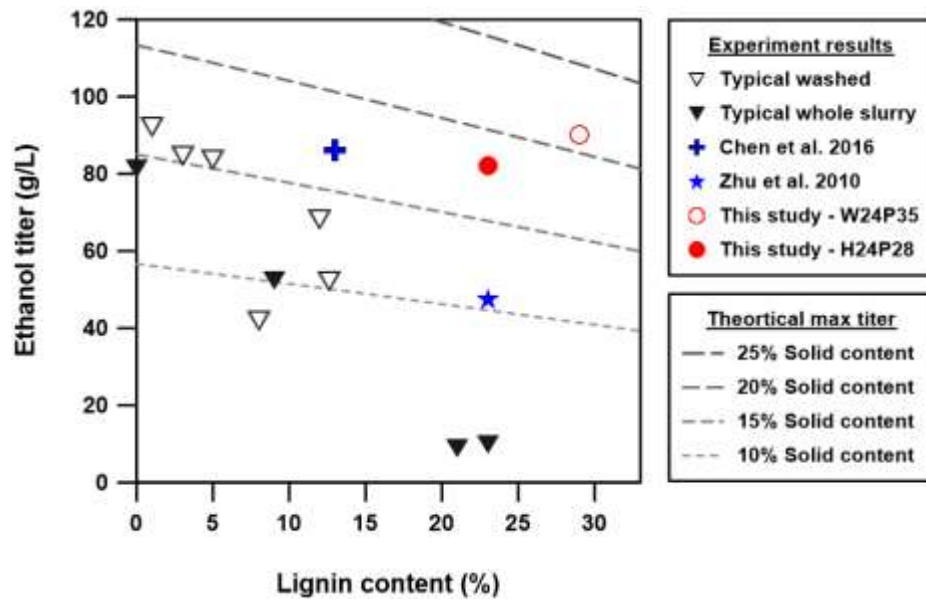
Fig. 5.6 Impacts of lignin residues to ethanol titer of different feedstock and biorefinery processes. The dashed lines show the maximum ethanol titers that can be obtained at different solid loads, and the spots show some examples from literature and this study for comparison.
