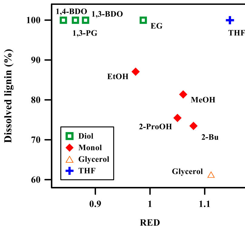
Fig. 6.7 Solubility test with different relative energy difference (REDs) between lignin and solvents under three conditions.
