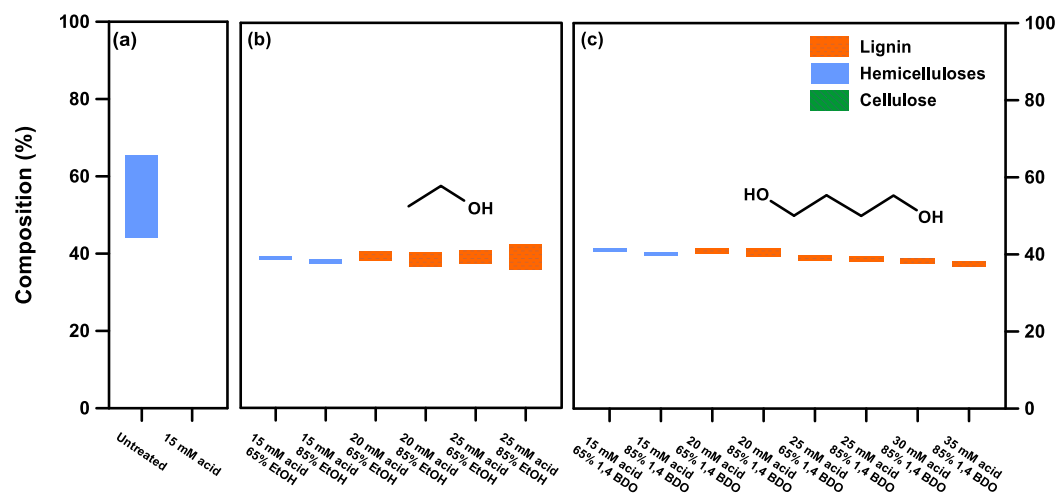
Fig. 6.3 Chemical compositions of DA, EtOH and 1,4-BDO pretreated eucalyptus.
