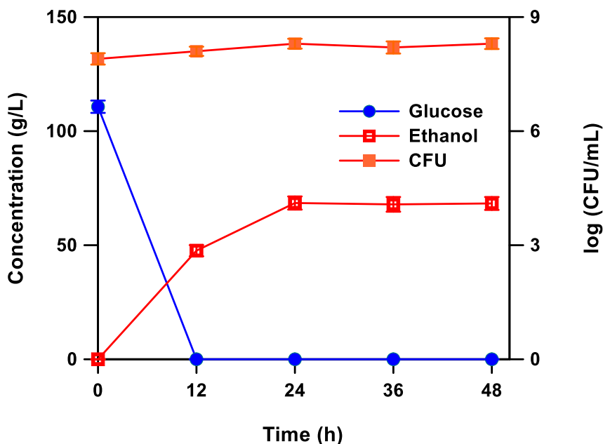
Fig. 4.2 Time course for SSF process using the washed substrate at 20% (w/w) solid loading. Symbols: closed circles, glucose concentration; opened squares, ethanol concentration; closed squares, CFU. Data points represent the mean values from three independent experiments.
