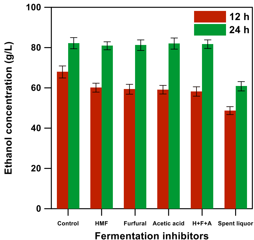
Fig. 4.3 Ethanol production formation by Saccharomyces cerevisiae during the fermentation of synthetic mediums and pretreatment spent liquor. H+F+A, HMF, Fufural and Acetic acid. Data points represent the mean values from three independent experiments.
