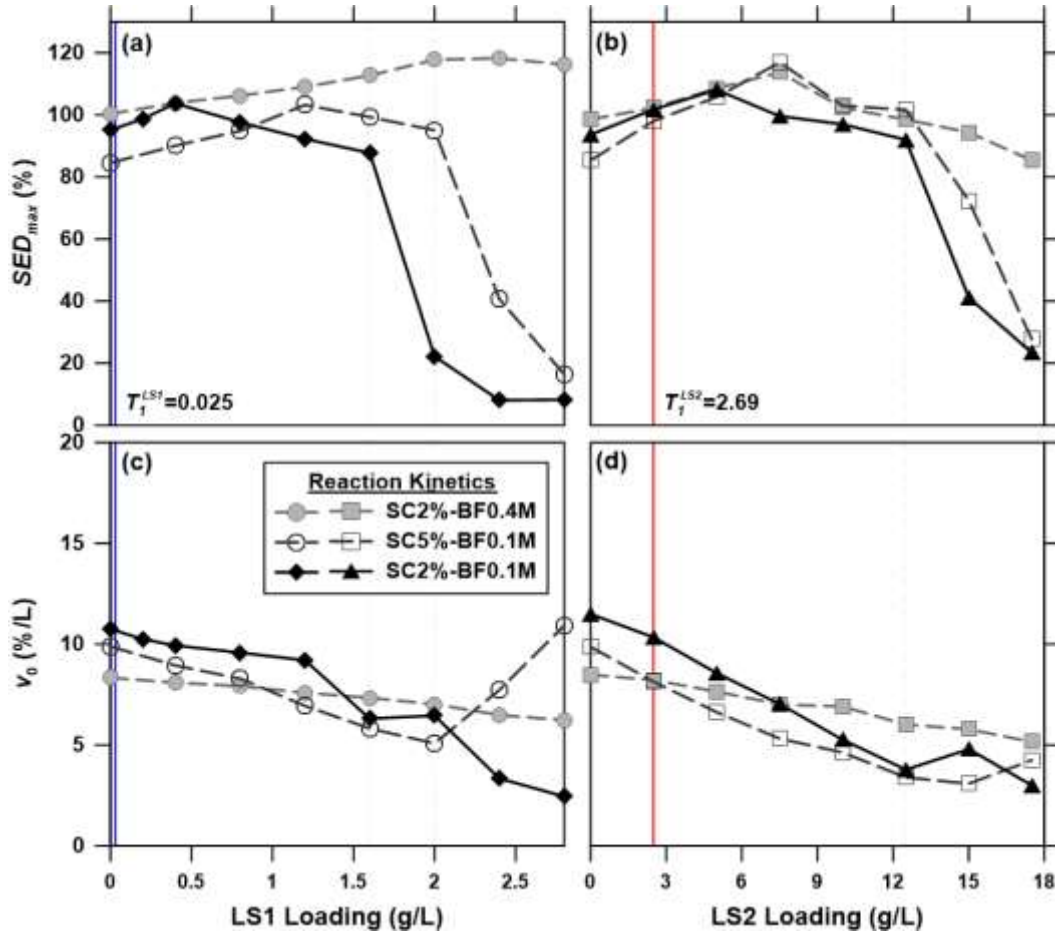
Fig. 3.6 Effects of LS1 (a, c) and LS2 (b, d) on enzymatic digestibility of SP10W substrate. SC: substrate content and BF: acetate buffer concentration, respectively.
