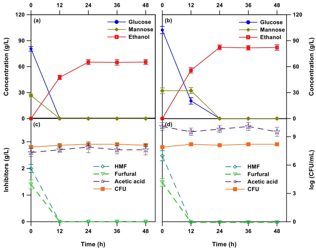
Fig. 4.5 Time course for SSF process using the whole slurry at 20% (w/w, a and c) and 25% (w/w, b and d) unwashed solid loading. Symbols: closed circles, glucose concentration; closed rhombus, mannose concentration; opened squares, ethanol concentration; opened rhombus, HMF concentration; opened inverted triangles, furfural concentration; opened pentagrams, acetic acid concentrations; closed squares, CFU. Data points represent the mean values from three independent experiments.
