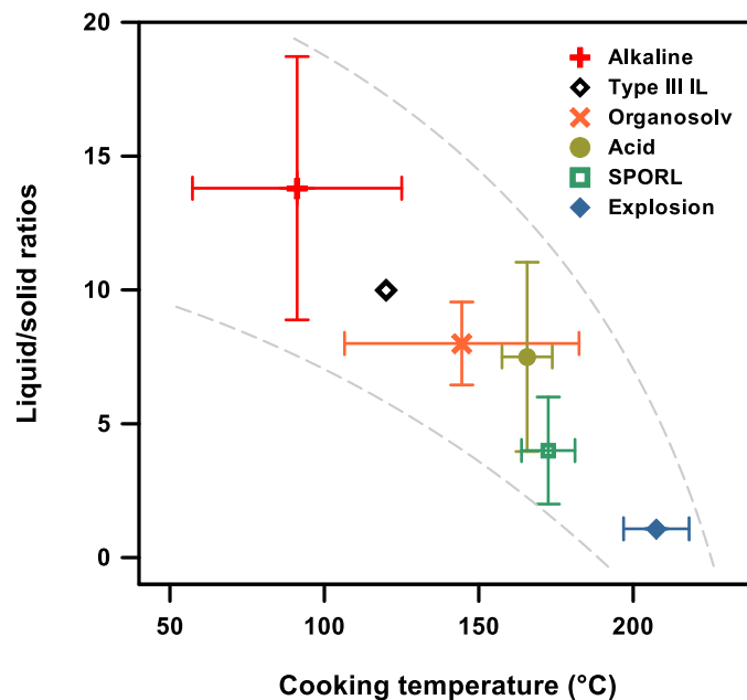
Fig. 2.10 Liquid/solid ratios of published pretreatment processes as a function of treatment temperature. Water (with co-solvent) consumption reduced with increased temperature.
