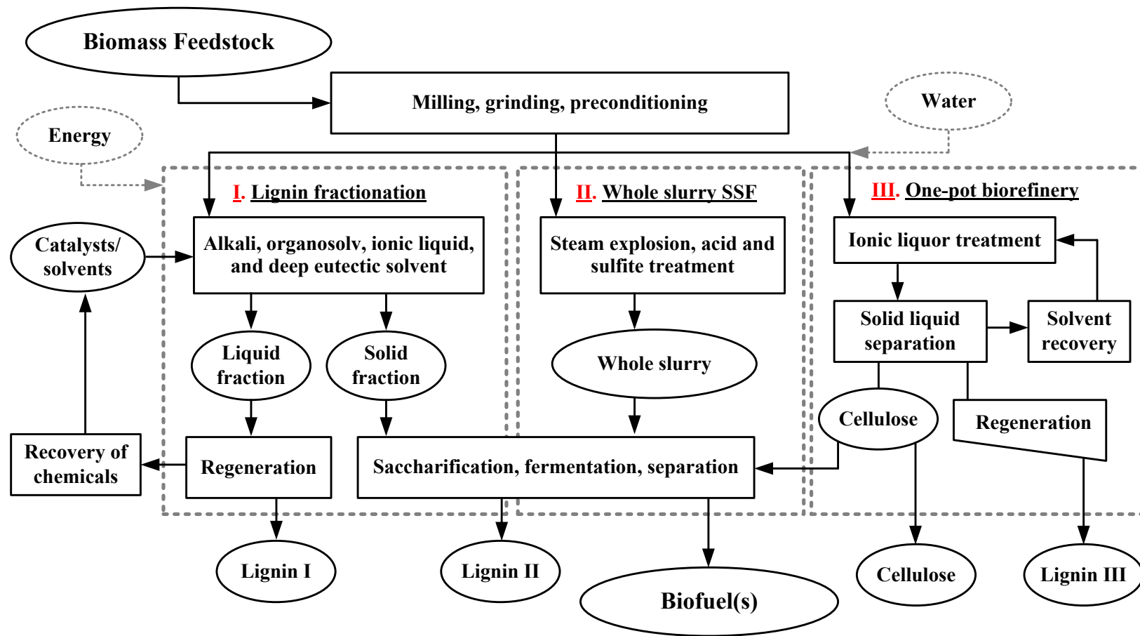
Fig. 2.5 Three biorefinery concepts for complete utilization of lignocellulosic biomass in bioenergy system.
