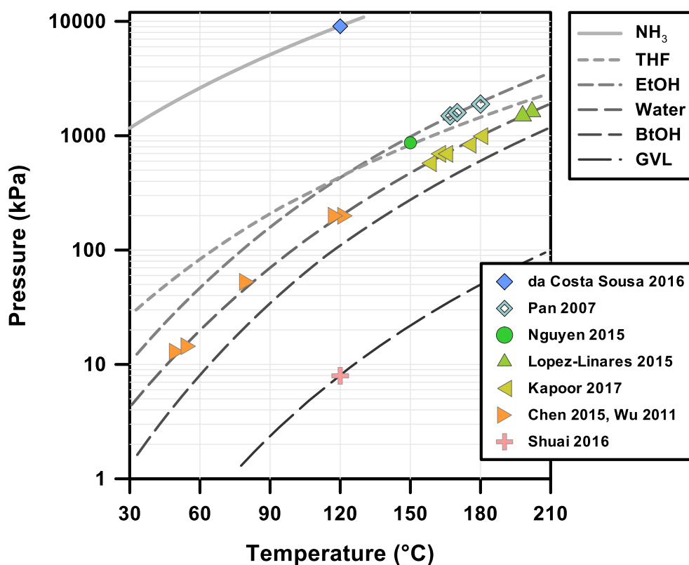
Fig. 2.9 Temperature-pressure relationships (curves) of different solvents for biomass pretreatment. Symbols represent the practical ranges of pretreatment temperatures used in published studies. Note: the pressures were presented in log scale.
