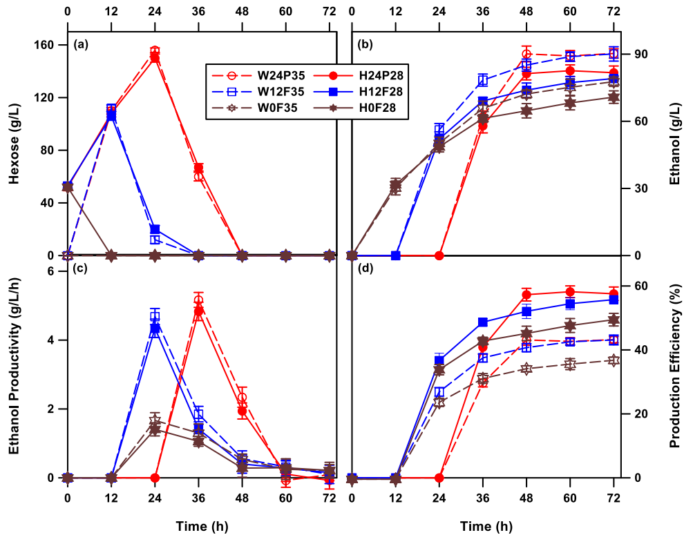
Fig. 5.4 Changes of hexose (a), ethanol (b), ethanol productivity (c) and bioconversion efficiency (d) of different fed-batch PSSF processes over time.
