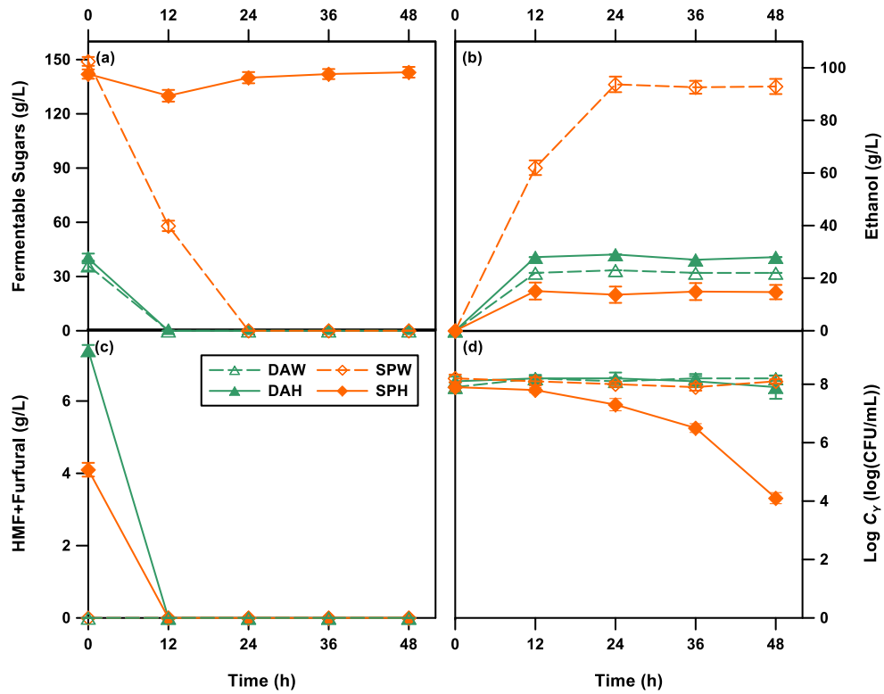
Fig. 5.2 Changes of hexose (a), ethanol (b), HMF+furfural (c) and CFU (d) of SSF over time. DAW: diluted acid pretreated washed slurry; DAH: diluted acid pretreated whole slurry; SPW: sulfite pretreated washed slurry and SPH: sulfite pretreated whole slurry.
