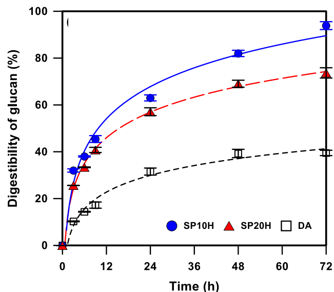
Fig. 3.1 Effects of sulfite loading on the enzymatic digestibility (SED) of sulfite pretreated substrates. Substrate content and acetate buffer concentration are 2% (w/v) and 0.1 M, respectively. H: whole slurry.
