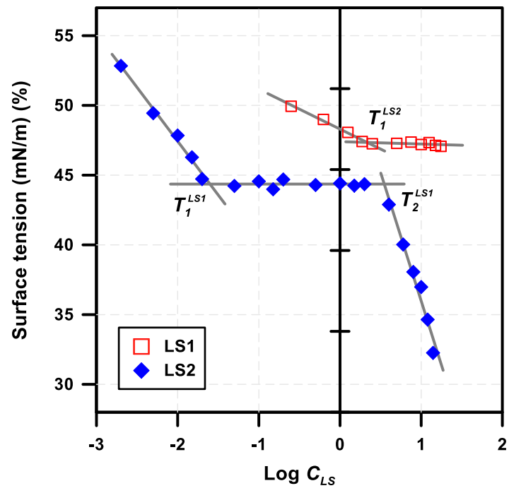
Fig. 3.2 Surface tension-concentration isotherm for two lignosulfonates. T_1 : critical aggregation concentrations; T_2 : critical micelle concentration.
