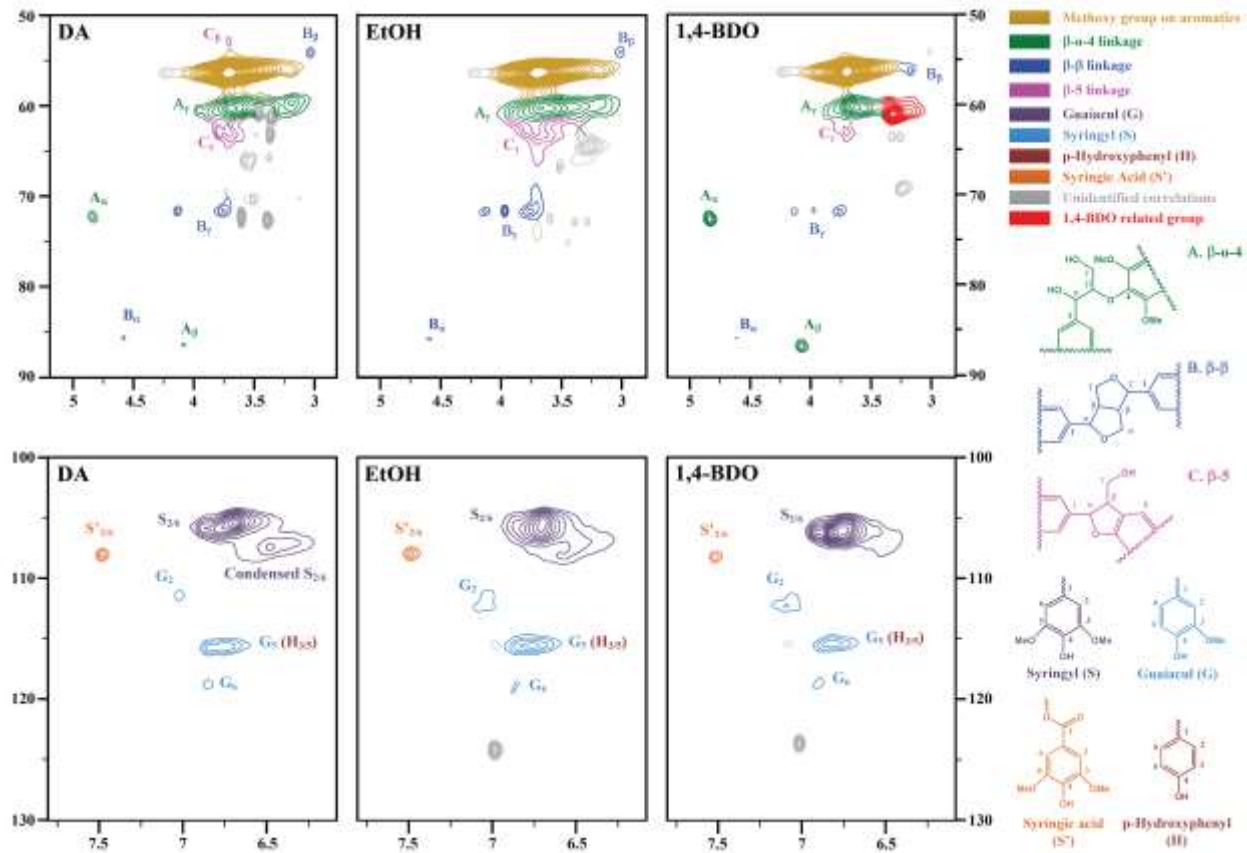
Fig. 6.4 2D HSQC NMR spectra of DA (15 mM acid), EtOH (15 mM acid and 65% EtOH) and 1,4-BDO (15 mM acid and 65% 1,4-BDO) residual lignin.
