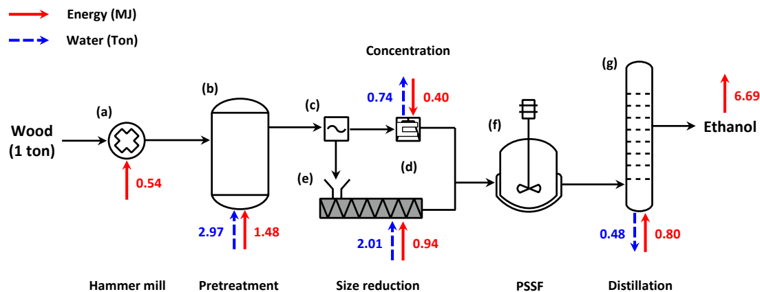
Fig. 5.1 Flow diagram of the water and energy balances of different unit processes in the proposed biorefinery for conversion of 1 ton softwood feedstock in ethanol.
