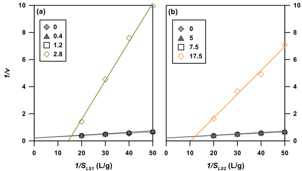
Fig. 3.4 Kinetic analysis of SP10W substrate enzyme hydrolysis in the presence of several concentrations of the inhibitor at different substrate concentrations. LS1: (a); LS2: (b). The legend represents the dosages (g/L) of LS. v : initial rate of enzymatic hydrolysis; [S] : substrate concentration (w/w, %).
