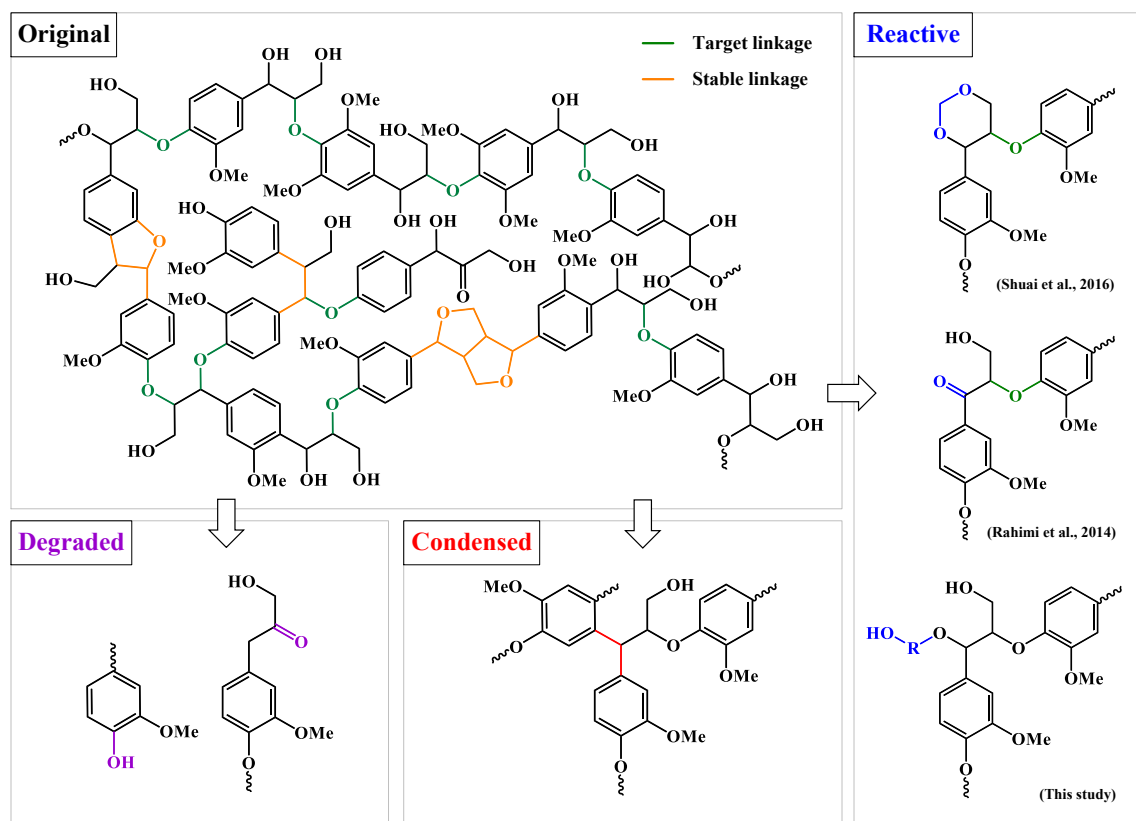
Fig. 6.1 Types of linkages in lignin structure before and after pretreatment.
