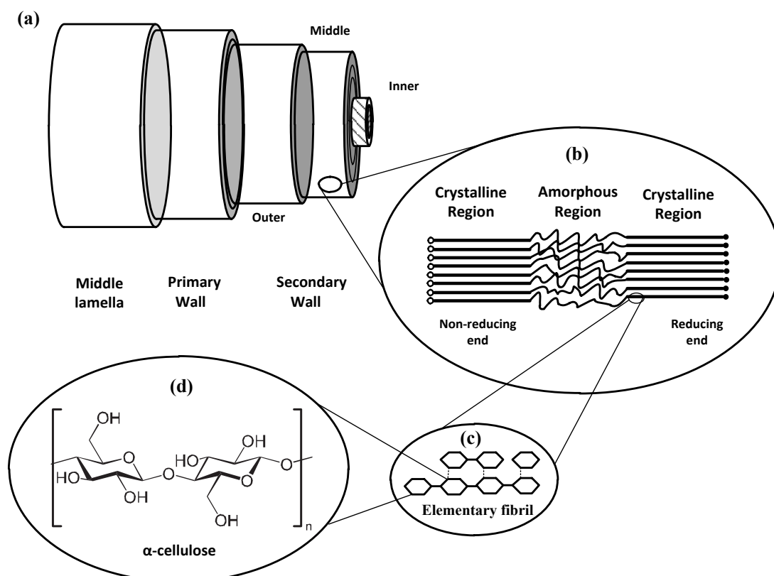
Fig. 2.1 Scheme of cellulose in plant cell (a) plant cell wall; (b) cellulose molecular chains within the crystalline region of cellulose microfibril; (c) elementary fibril and (d) two \alpha -cellulose. Note: the dimension of the cell wall is not in scale, the direction of microfibrils alignment is not based on real image. This diagram was re-plotted based on Anderson and Kerr (1938) and Gordon and Hsieh (2006).
