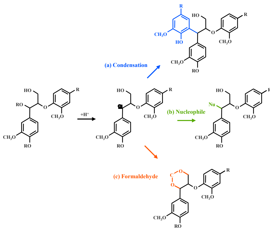
Fig. 2.8 Condensation or stabilization of dissociated lignin.
