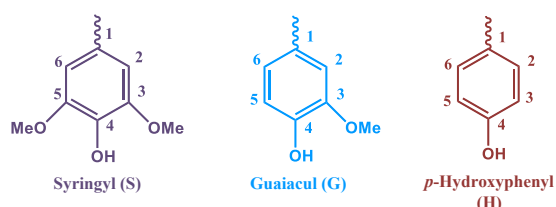
Fig. 2.3 The three building blocks of lignin (Chakar & Ragauskas, 2004).
