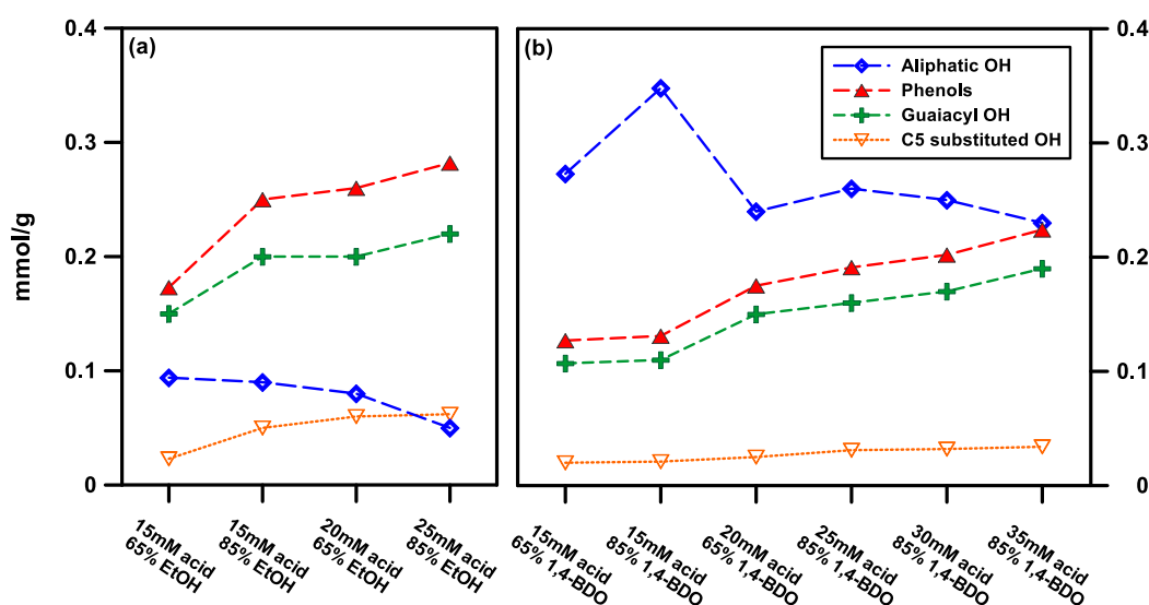
Fig. 6.6 Hydroxyl groups of soluble lignin at different pretreatment severities using EtOH and 1,4-BDO.
