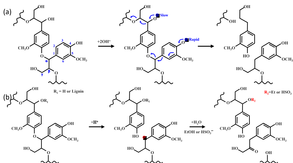
Fig. 2.7 (a) Cleavage of \alpha -O-4 and \beta -O-4 bonds in alkaline pretreatment process; (b) cleavage of \alpha -O-4 and \beta -O-4 bonds in dilute acid, organosolv, and sulfite pretreatment (SPORL) processes.
