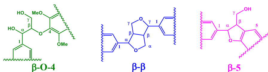
Fig. 2.4 Example linkages between phenylpropane units in lignin.
