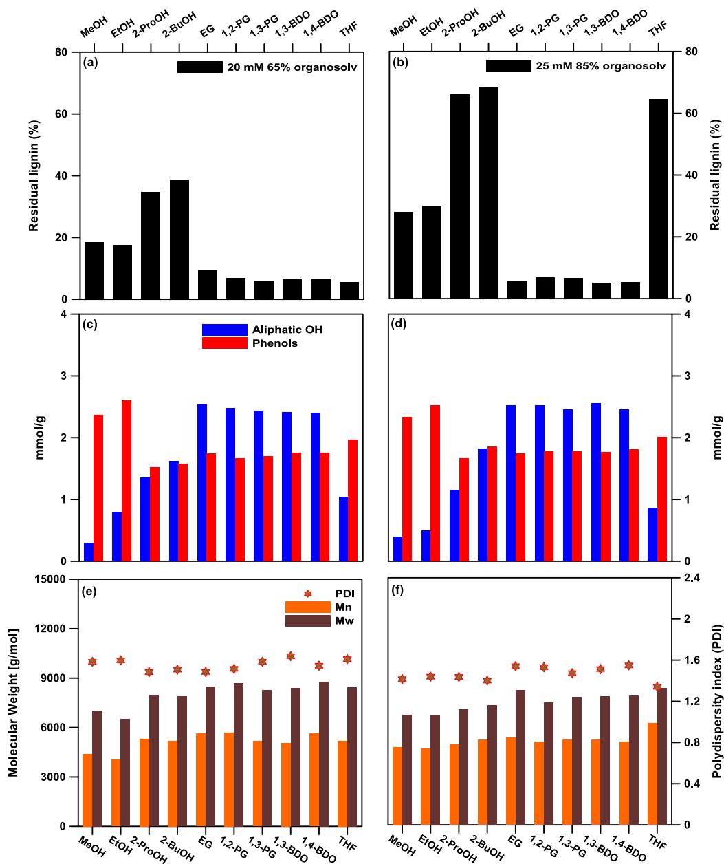
Fig. 6.8 Effects of organosolv pretreatments on isolated lignin yields and lignin structure integrity among different solvents. (a) and (b) percentage of residual lignin after organosolv pretreatments at two severities; (c) and (d) hydroxyl group contents of organosolv soluble lignin; (e) and (f) Molecular weights and polydispersity index of organosolv soluble lignin.
