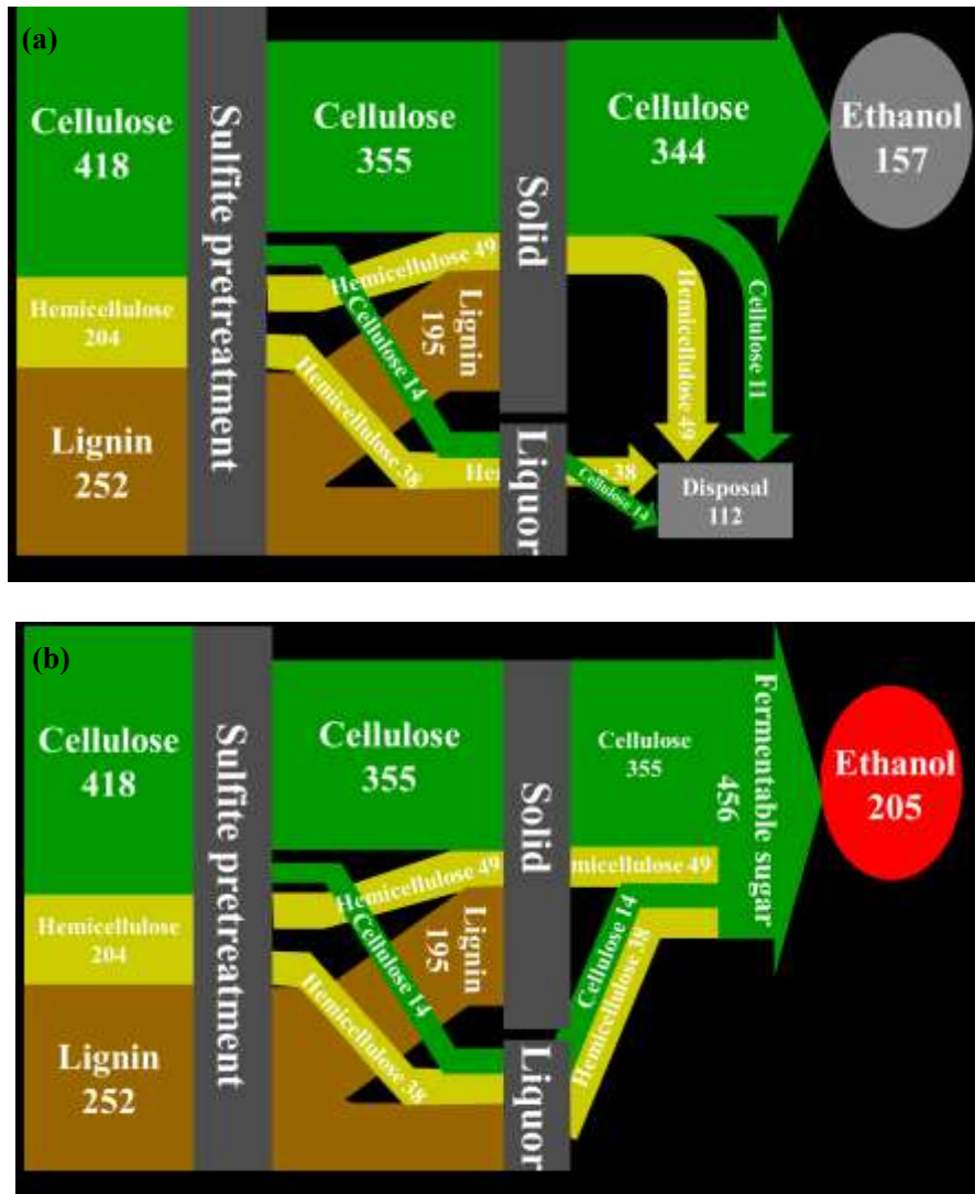
Fig. 4.6 Block diagram showing component mass balance (unit = kg). (a) washed substrate; (b) the whole slurry.
