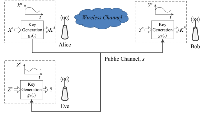
Fig. 3. Key generation model
