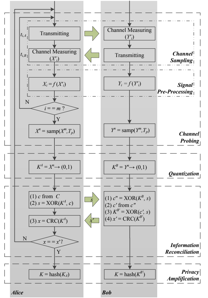
Fig. 4. Key generation procedure
