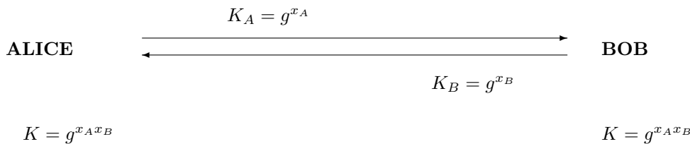
Figure 1. The Diffie Hellmann protocol
