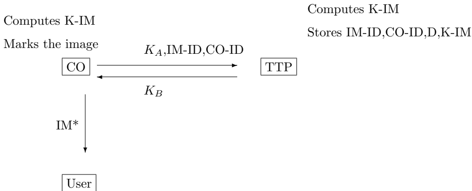
Figure 2. A scheme for watermarking images with the Diffie-Hellman protocol
