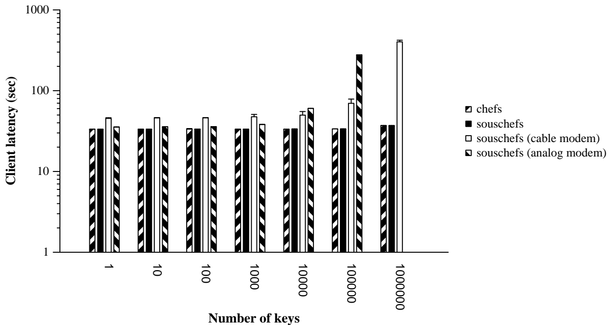
Figure 9: A log-log chart of single client latency to read 10 000 8 KB encrypted files and the associated content keys. Key regression maintains a constant client latency regardless of the number of keys. Under low-bandwidth, high-latency conditions, Sous-Chefs latency is dominated by the transfer time of keys after reaching 10 000 keys. Key regression enables much better latency in Chefs.
