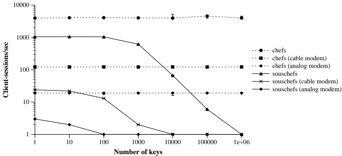
Figure 8: Aggregate publisher throughput for key distribution plotted on a log-log graph. A client-session consists of fetching key material sufficient to generate all the keys to decrypt the published content. Key regression enables a publisher to support many client-sessions per second. Chefs always performs better than Sous-Chefs because key regression performance is effectively independent of the rate of membership turnover.
