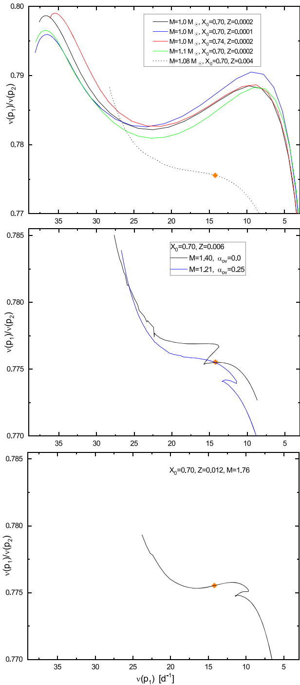
Figure 6. Petersen diagrams spanning from the ZAMS to the immediate post-main-sequence phase of evolution for various metallicity values in our grid. In each panel, the location of the best model is indicated by the orange diamond. The observed frequency ratio of \nu_1/\nu_2 for KIC 5950759 clearly excludes low metallicities (i.e. Z < 0.003 ).
