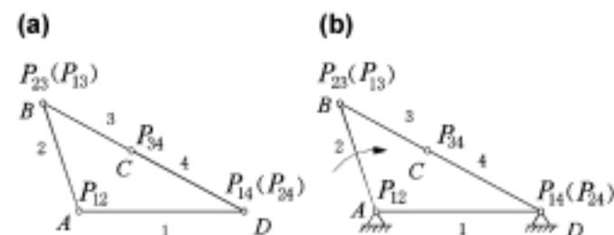
Figure 7. Instant inactive joint of four-bar mechanism ( P is instant velocity center; subscripts represent the number of bars): (a) four-bar kinematic chain and (b) four-bar mechanism with link 1 fixed.
