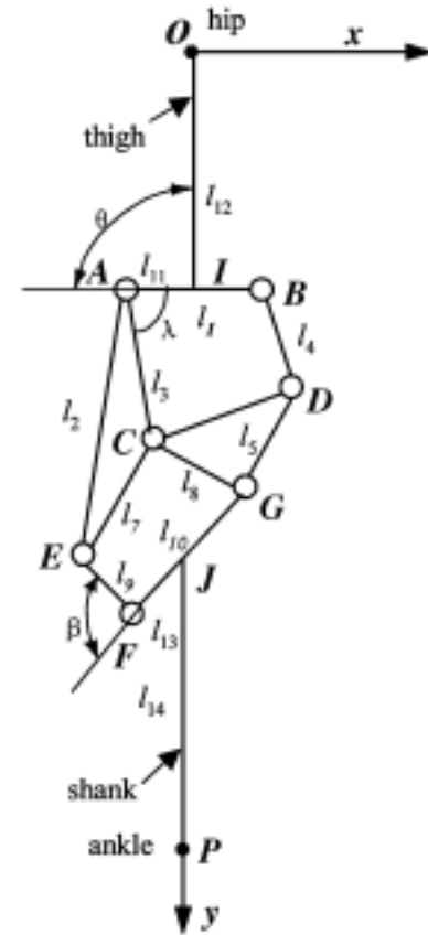
Figure 3. Design parameters for optimization.
