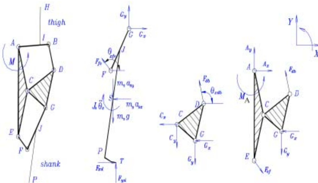
Figure 9. Free body diagram of six-bar mechanism when torque applied on joint A.
