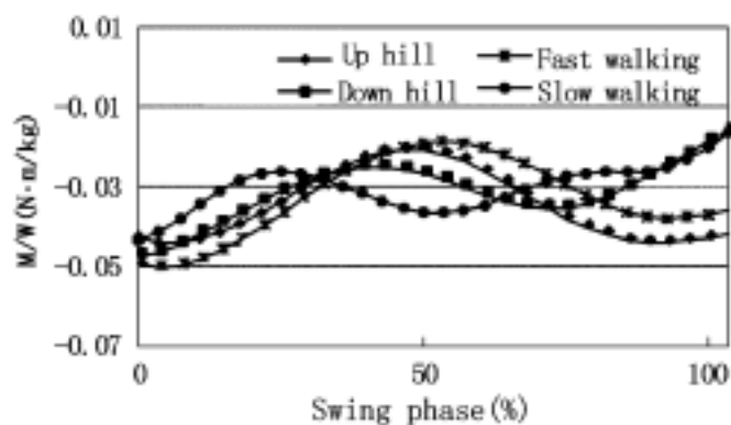
Figure 13. Moments provided by controllable damper.
