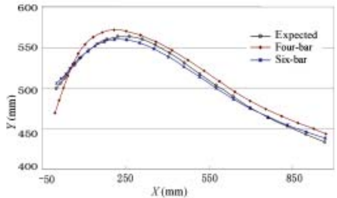
Figure 5. Comparison of ankle joint trajectory in swing phase between different mechanisms.
