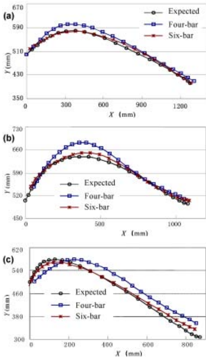
Figure 6. Trajectory of ankle joint in swing phase in different walking pattern: (a) fast walking, (b) up hill, and (c) down hill.
