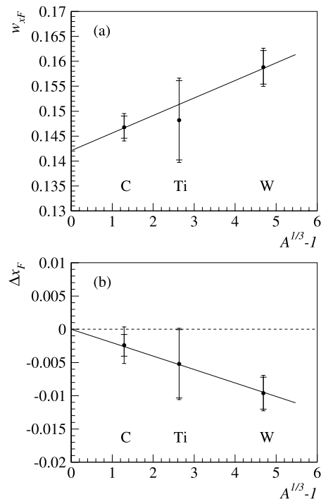
Fig. 4.6 The width (a) and shift (b) of the J/\psi x_F distributions as a function of A^{1/3} - 1 (see (4.5) and (4.6)). The double error bars represent total and statistical uncertainties. The data are fitted with linear functions
