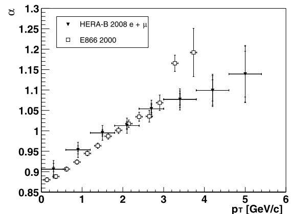
Fig. 5.1 The nuclear suppression parameter \alpha as a function of p_T measured by HERA-B (filled triangles, plotted with total and statistical uncertainties) and by E866 [7] (empty squares)
