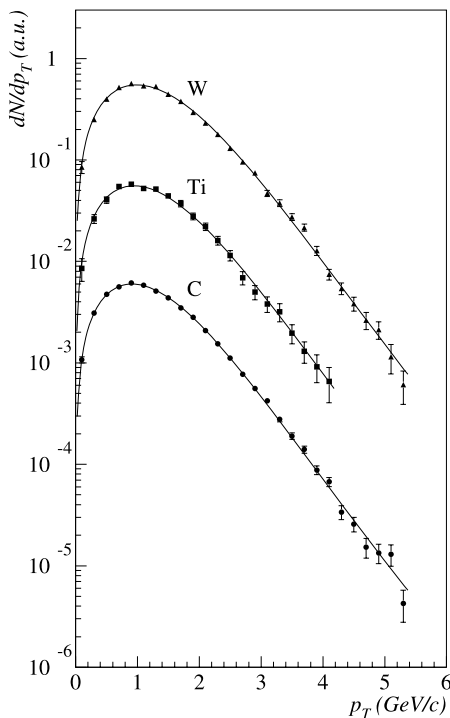
Fig. 4.1 Inclusive p_T distributions of J/\psi mesons for three target materials with arbitrary normalizations. For visibility, the scales are shifted arbitrarily. The error bars represent the combination of statistical and systematic uncertainties. The interpolating lines are the results of a simultaneous fit of the three p_T distributions to (4.2) performed with the method described in Sect. 4.2
