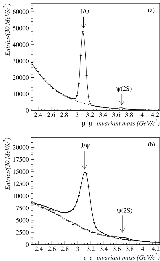
Fig. 3.1 The \mu^+\mu^- (a) and e^+e^- (b) invariant mass distributions for the full data sample in the J/\psi mass region. The continuous lines represent the result of fits performed with the functions described in the text; the dashed lines are the fitted backgrounds. The histogram in (b) represents the background shape as determined from combinations of tracks reconstructed in different events
