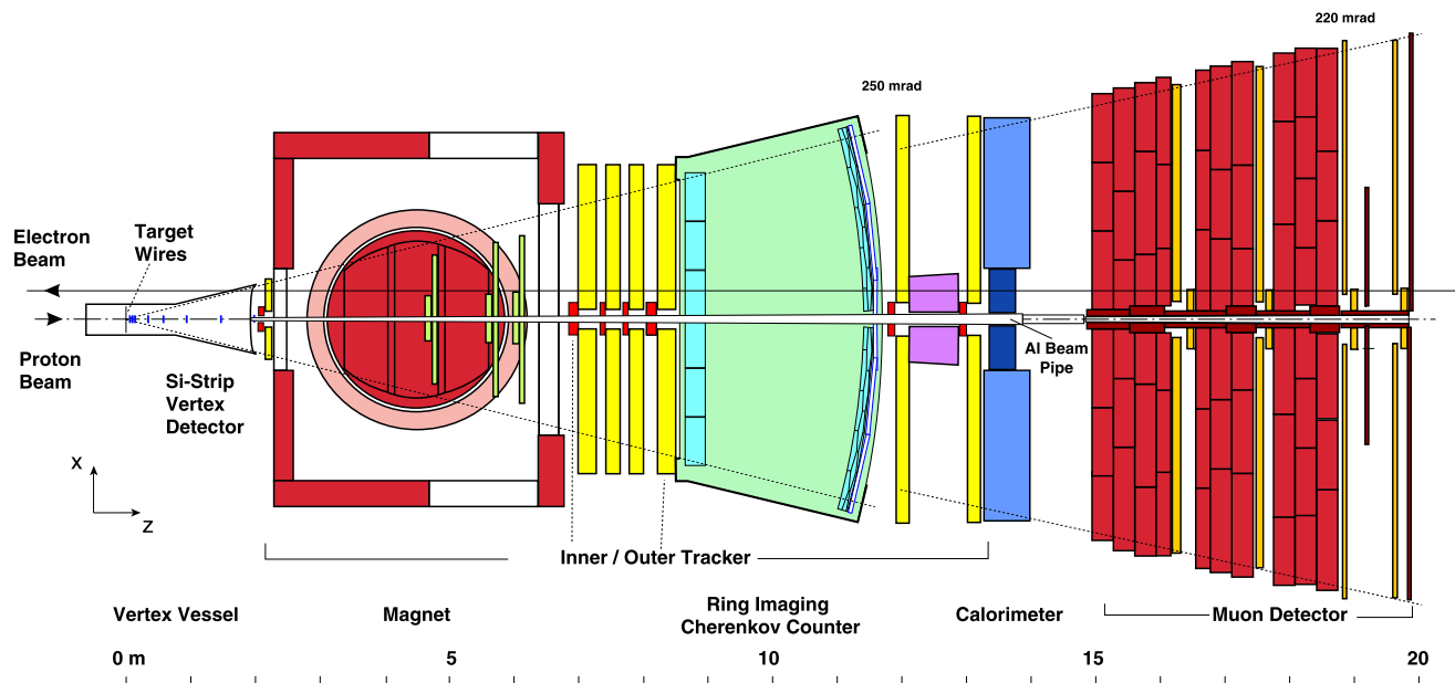
Fig. 2.1 Top view of the HERA-B detector
