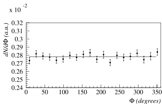
Fig. 4.3 Distribution of the azimuthal production angle of the J/\psi s fitted to a constant. The error bars include only statistical contributions
