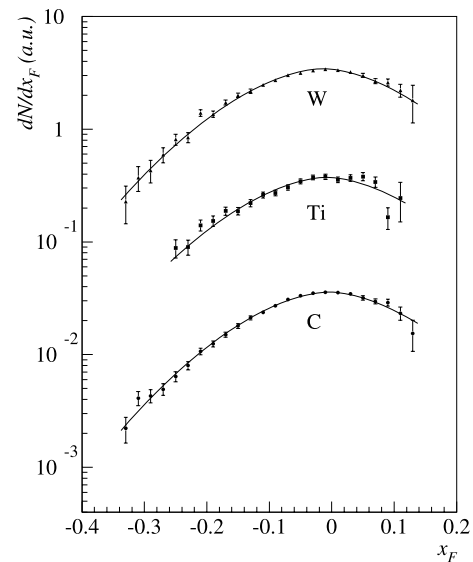
Fig. 4.2 Inclusive x_F distributions of J/\psi mesons for the three target materials with arbitrary normalizations. For visibility, the scales are shifted arbitrarily. The error bars represent the combination of statistical and systematic uncertainties. The interpolating lines are the results of a simultaneous fit of the three x_F distributions to (4.3) performed with the method described in Sect. 4.2
