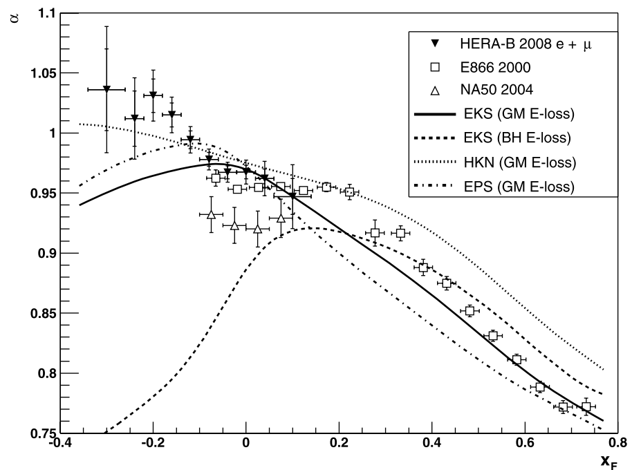
Fig. 5.2 Measurements of \alpha as a function of x_F by HERA-B (filled triangles, plotted with total and statistical uncertainties), E866 (empty squares) and NA50 (empty triangles). The curves were calculated by Vogt [10, 11] based on three different nuclear parton distribution functions: (EPS [49], EKS [43, 51] and HKN [50]) and two models of initial state energy-loss: BH [13] and GM [13]. For all approaches, energy loss, intrinsic charm and shadowing are taken into account
