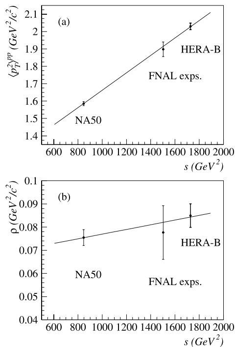
Fig. 4.5 Energy dependence of the parameters \langle p_T^2 \rangle^{pp} (a) and \rho (b) as defined in (4.4) describing the p_T -broadening of the J/\psi . The points represent the results obtained by HERA-B (black filled circles, with total and statistical uncertainties), at Fermilab [3–6] and at the SPS [8, 9]. The data are fitted with linear functions
