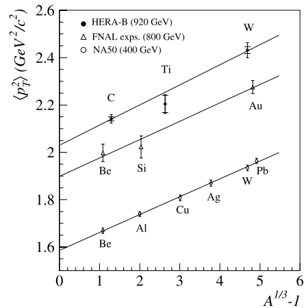
Fig. 4.4 The \langle p_T^2 \rangle of the produced J/\psi s as a function of A^{1/3} - 1 (see (4.4)). The results of the present analysis (black filled circles with total and statistical uncertainties) are compared to previous measurements performed with different beam energies at Fermilab [3–6] and at the SPS [8, 9]. The data are fitted with linear functions
