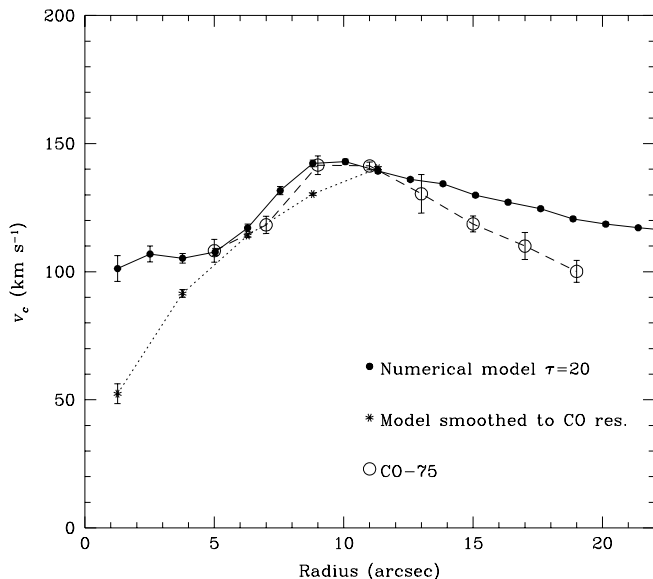
FIG. 14.—Gas rotation curve as derived from the numerical velocity field of Fig. 13 (filled dots, drawn line). Also shown is the SPH curve smoothed to the CO resolution (stars, dotted line). CO-75 (see Fig. 8) is shown for comparison. Due to variable resolution, in the model, the CO-75 curve should be compared to smoothed CO for less than 10'' and to unsmoothed CO for more than 10'' .
