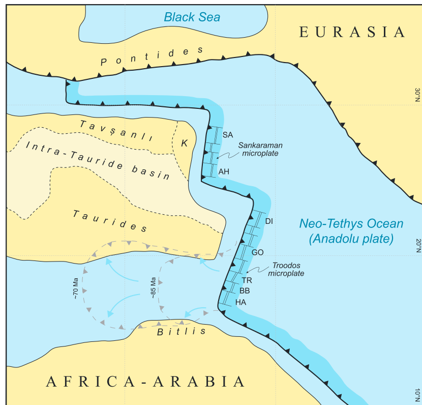
Figure 8. Paleogeographic reconstruction of the eastern Mediterranean Neo-Tethys soon after subduction initiation (~95 Ma) showing the main subduction zones. The dark blue shaded area adjacent to the trench in a fore-arc position indicates the source area of the suprasubduction zone ophiolites. The proposed eastward invasion of the southeastern subduction segment at ~85 and ~70 Ma is shown. The blue arrows indicate the transport directions of ophiolites from the Troodos microplate toward the southern margin of the Tauride (Göksun ophiolite) and the northern margin of Gondwana (Troodos, Baer-Bassit, and Hatay ophiolites). K, Kırşehir block. SA, Sarkaraman ophiolite. AH, Alihoca ophiolite. DI, Divriği ophiolite. GO, Göksun ophiolite. TR, Troodos ophiolite. BB, Baer-Bassit ophiolite. HA, Hatay ophiolite.
