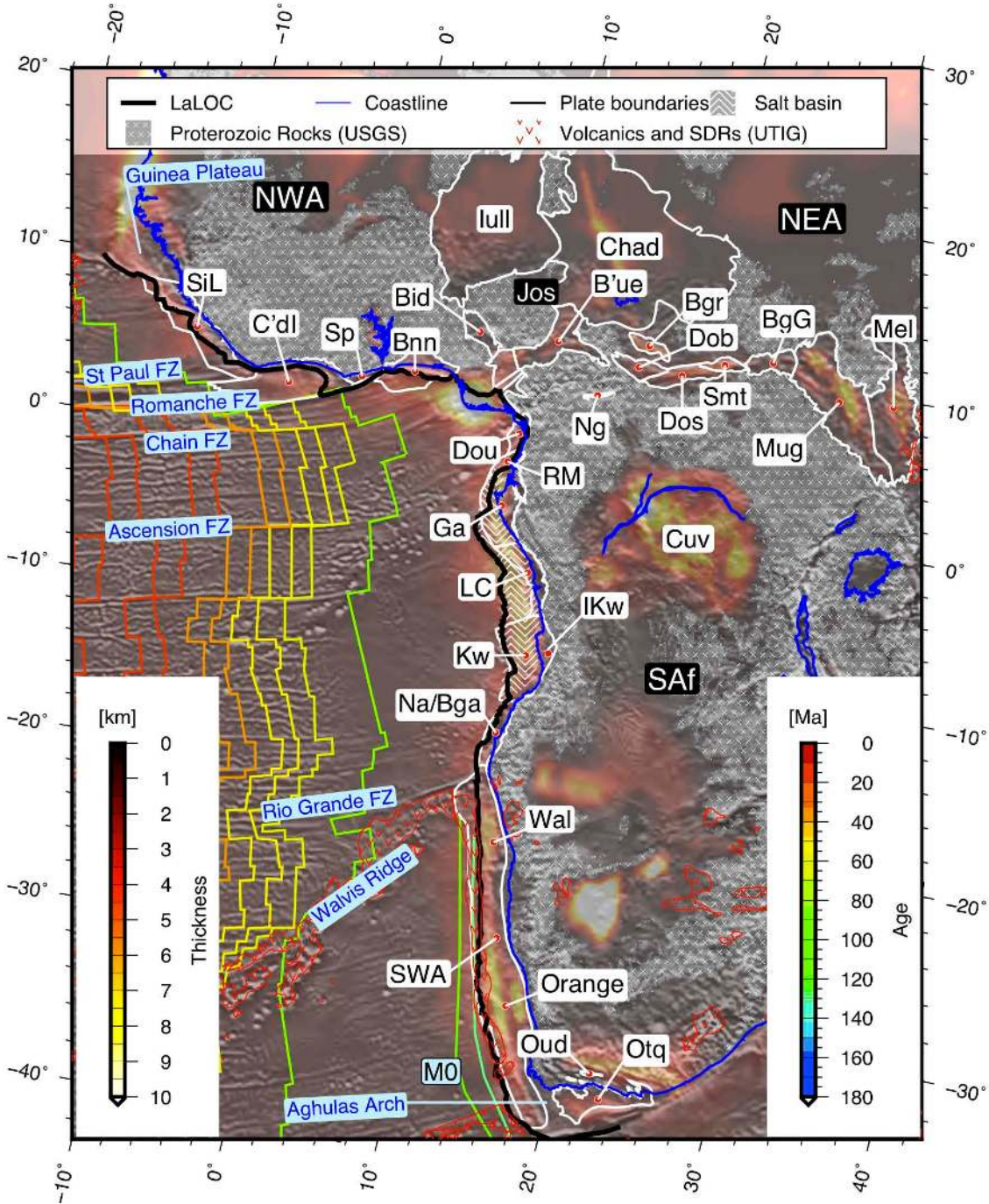
Fig. 5. Oblique Mercator map of present-day Africa, with onshore topography (ETOPO1; Amante and Eakins, 2009), offshore free-air gravity (Sandwell and Smith, 2009), both greyscale, and gridded sediment thickness (Exxon Production Research Company, 1985) superimposed. Map legend: LaLOC – landward limit of oceanic crust, Proterozoic rocks and Mesozoic extrusive rocks based on United States Geological Survey (2012). Seaward-dipping reflectors (SDRs) based on UTIG PLATES open data ( https://www.ig.utexas.edu/research/projects/plates/data.htm ). White polygons indicate sedimentary basins (N to S): SiL – Sierra Leone marginal; C'dI – Côte d'Ivoire marginal; Sp – Saltpond; Bnn – Benin; Bid – Bida; Iull – Iullemmeden; Chad – Chad Basin; B'ue – Benue Trough; Bgr – Bongor Trough; Dob – Doba; Dos – Doseo; BgG – Banggara Graben; Mel – Melut; Mug – Muglad; Smt – Salamat; Ng – Ngaoundere; Dou – Douala; RM – Rio Muni; Ga – Gabon coastal; Cuv – Cuvette central; LC – lower Congo; Kw – Kwanza/Cuanza; IKw – inner Kwanza; Na/Bga – Namibe/Benguela; Wal – Walvis; SWA – southwest African marginal; Orange – Orange; Oud – Oudtshoorn; Otq – Outeniqua. Fz: oceanic fracture zone. Coloured lines are oceanic isochrons from Müller et al. (2008); M0 – M0 magnetic anomaly (120.6 ma). Plates and sub-plates: NWA – northwest Africa; NUB – Nubia/northeast Africa; JOS – Jos Plateau sub-plate; and SAf – austral Africa. Origin of map projection at 10° S, 5° W; azimuth of oblique equator 80°.
