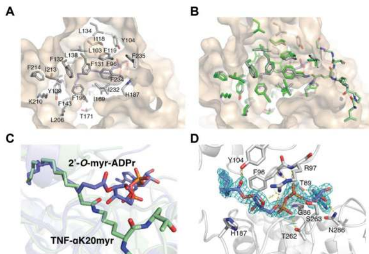
Figure 8. Comparison of SIRT2 – 2'-O-myristoyl-ADPr with SIRT2 – TNF \alpha -K20myr structure A , hydrophobic pocket in SIRT2 that accommodates the myristoyl chain of 2'-O-myristoyl-ADPr. B , superimposition of SIRT2 – 2'-O-myristoyl-ADPr (grey) and SIRT2 – TNF \alpha -K20myr (green) structures highlighting the hydrophobic residues in the myristoyl chain binding site. C , overlay as in B highlighting differences in myristoyl chain between substrate and product. D , 2F_o - F_c omit electron density map (blue mesh, 1\sigma ) of 2'-O-myristoyl-ADPr molecule and hydrogen bonding network surrounding 2'-O-myristoyl-ADPr. Also shown is the catalytic histidine residue.
