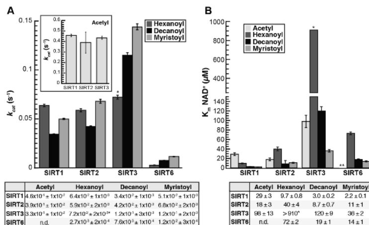
Figure 2. k_{cat} and K_m, NAD for SIRT1, SIRT2, SIRT3, and SIRT6 deacylation reactions A, k_{cat} , inset: k_{cat} for acetylated substrate plotted separately for clarity; Calculated k_{cat} values determined from non-linear regression fits to Michaelis-Menten shown below ( n \geq 3 , \pm standard deviation). *Estimate for SIRT3 resulting from inability to saturate reaction with NAD^+ . B, K_m for NAD^+ , Calculated K_m, NAD values determined from non-linear regression fits to Michaelis-Menten shown below. *Estimate for SIRT3, ** K_m, NAD with acetylated peptide for SIRT6 was not measured due to prohibitively high peptide substrate necessary to saturate the reaction ( n \geq 3 , \pm standard deviation of mean).
