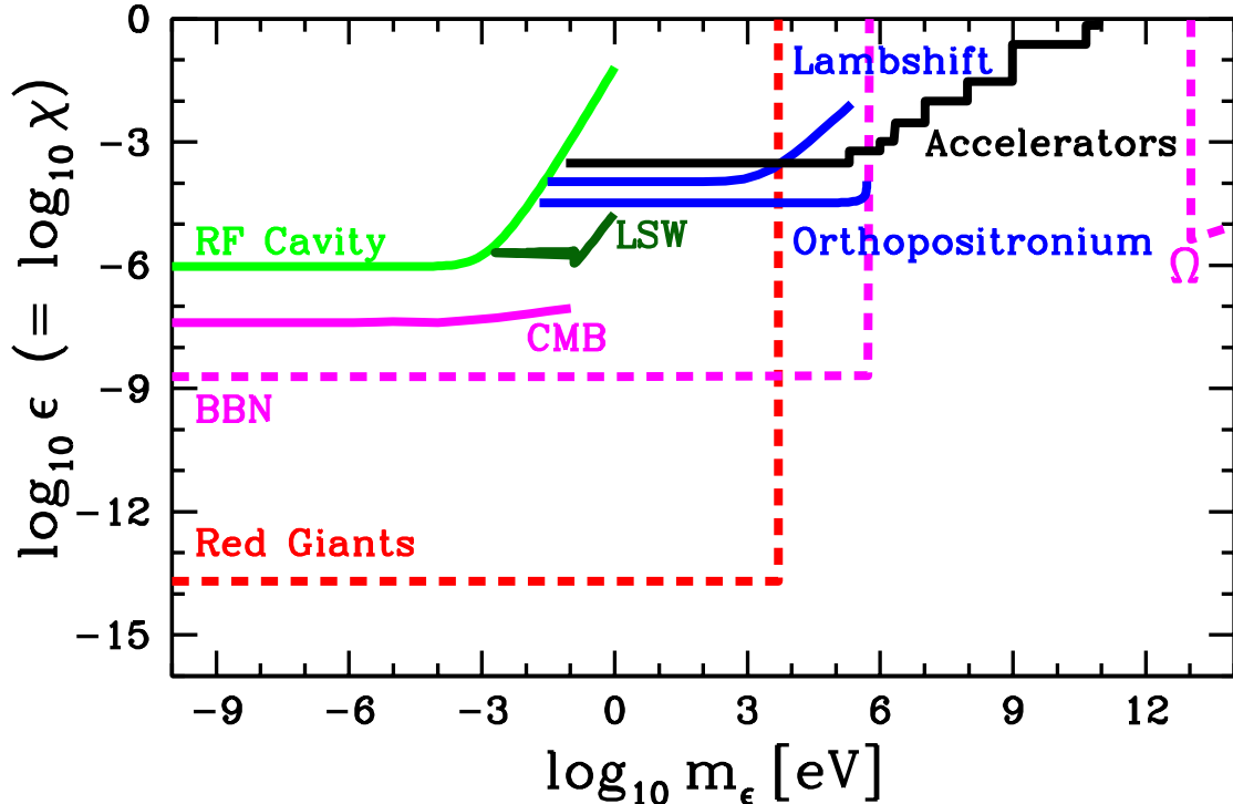
Figure 2: Upper limits on the fractional charge \epsilon = Q_\epsilon/e of a hidden-sector fermion with mass m_\epsilon . Some of the limits only apply if there is also an ultralight hidden-sector U(1) gauge boson which gives rise to the minicharge \epsilon \sim \chi by gauge kinetic mixing with the photon. Laboratory limits arise from laser polarization and light-shining-through-a-wall (LSW) experiments [30], from energy loss considerations of RF cavities [36], from searches for the invisible decay of orthopositronium [37], from Lamb shift measurements [38] and from searches at accelerators [39, 40]. Limits from cosmology are due the non-observation of a significant distortion of the spectrum of the cosmic microwave background (CMB) radiation [41] (for a limit exploiting the CMB anisotropy, see Ref. [42]), due to the apparent successfullness of standard big bang nucleosynthesis (BBN) [43], and due to the observational requirement that the contribution of MCPs to the energy density should not overclose the universe, \Omega = \rho/\rho_{\text{crit}} < 1 [44]. Finally, an astrophysical limit can be placed by energy loss considerations of red giants [43].
