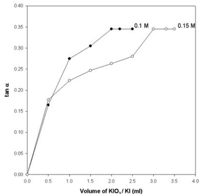
Figure 3. Effect of the volume of (A) 0.10 M potassium iodate, (B) 0.15 M potassium iodide on the initial rate of reaction.
