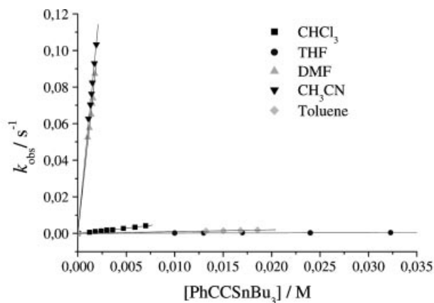
Figure 2. Plots of k_{\text{obs}} versus the stannane concentration for the transmetalation of 1c with \text{PhC}\equiv\text{CSnBu}_3 in different solvents at 25 °C in the presence of fn ( [\mathbf{1c}]_0 = 1 \cdot 10^{-4} M; [\text{fn}] = 2 \cdot 10^{-4} M)
