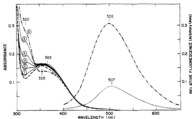
FIGURE 4: Inactivation of reduced lactate oxidase with 2-keto-3-butyrate. An anaerobic solution (2.0 ml) containing lactate oxidase, 3.4 \times 10^{-5} M in 0.01 M imidazole-HCl, pH 7.0, lactate dehydrogenase (0.264 mg), and 5 \times 10^{-4} M oxalate was incubated in the dark until the spectral changes occurring upon binding of oxalate to lactate oxidase were complete ( \sim 15 min). This solution was then illuminated until complete formation of the N(5)-carbonate adduct of the flavin, and this species was allowed to decay to form the reduced flavin-enzyme complex ( \sim 24 h at 4^\circ\text{C} ): (---) absorption and (···) fluorescence emission spectrum. 2-Hydroxy-3-butyrate (30 \mu\text{l} of 0.8 M; final concentration, 1.2 \times 10^{-2} M) and 20 \mu\text{l} of 5 \times 10^{-1} M NAD + (final concentration, 5.0 \times 10^{-3} M) were then added anaerobically, and the same amounts of reagents were added to the reference cuvette. Curves 1, 2, 3, 4, 5, and 6 represent plots after 6, 18, 30, 58, 100 and 240 min, respectively, of incubation at 25^\circ\text{C} . The half-time of the reaction under these conditions is 50 min. (···) Represents the fluorescence emission of the inactivated enzyme excited at 370 nm and is corrected for the decay of the adduct (cf. text for further explanations).
