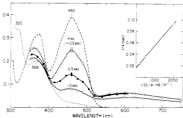
FIGURE 3: Spectral intermediates formed during the anaerobic reaction of lactate oxidase with 2-hydroxy-3-butynoate. The enzyme, 3.5 \times 10^{-5} M in 0.01 M imidazole-HCl, pH 7.0 (---), was mixed at 25 °C with solutions of DL-2-hydroxy-3-butynoate ( 5 \times 10^{-3} , 2 \times 10^{-3} , and 5 \times 10^{-4} M final concentration) in the same buffer. The curves shown, selected for illustration purposes, were obtained with 5 \times 10^{-3} M 2-hydroxy-3-butynoate: (□) at the end of first, fast phase; (●) at 0.5 s; and (○) at 1.0 s. (···) Represents the absorption at the end of the reaction and is identical with the spectrum of the inactivated enzyme. The inset shows the reciprocal plot of the first, fast rate of appearance of the long wavelength absorption measured at 580 nm at the concentrations of 2-hydroxy-3-butynoate given.
