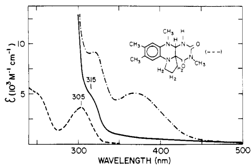
FIGURE 7: Reaction of the 2-hydroxy-3-butynoate-inactivated lactate oxidase with sodium borohydride. The enzyme (1.0 ml; 4.1 \times 10^{-5} M) was inactivated as described in Experimental Procedure and then passed through a short G25 column equilibrated with a buffer containing 10^{-2} M each of imidazole, Tris, and pyrazine and 4 \times 10^{-2} M \text{Cl}^- , pH 7.0 (---). To this solution at 25 °C were added aliquots (ca. 0.5 mg) of solid sodium borohydride over a period of 20 min until the absorption decrease at 370 nm was completed. A trace of 1-octanol was added to prevent excessive foaming. The pH of the solution at the end of reaction was \sim 9 (—). (---) Represents for comparison the spectrum of the model compound 3-methyl-4a,5-propano-4a,5,10a,1-tetrahydrolumiflavin (cf. structure), in 0.1 M KCl, at the same concentration.
