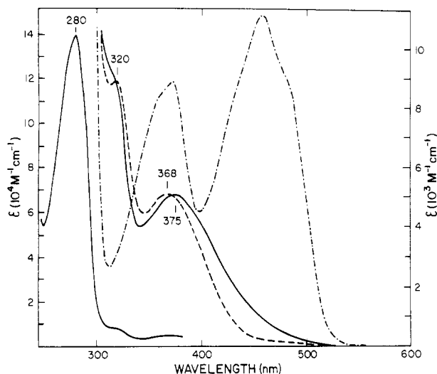
FIGURE 6: Spectral comparison of lactate oxidase after modification of the coenzyme with 2-hydroxy-3-butynoate (---); with 4a,5-propano-4a,5-dihydro-FMN bound to apolactate oxidase (—). Shows the absorption of the oxidized enzyme for comparison.
