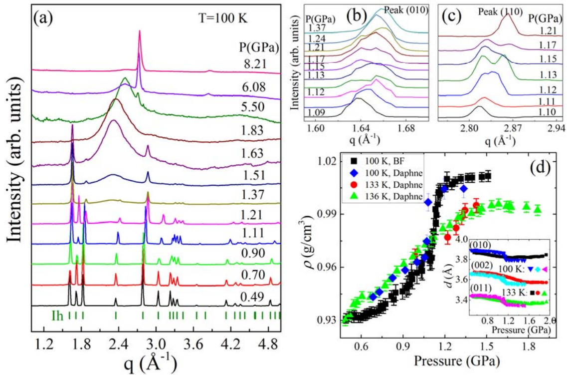
FIG. 1. (a) Structural evolution of compressed ice Ih at 100 K in quasi-hydrostatic condition using the ‘‘back-and-forth’’ approach [34]. The background was subtracted for the typical integrated x-ray diffraction patterns (Fig. S2). At 0.49 GPa, the diffraction pattern is indexed with hexagonal structure of ice Ih (Table S1). (b) and (c) the detailed structural evolutions of (010) and (110) reflections for crystalline ice Ih under compression. (d) Density of the crystalline phases as a function of pressure. The density is calculated using more than six indexed diffraction peaks. BF: back-and-forth approach. The inset in Fig. 1(d) shows pressure-dependent d -spacings of three typical diffraction reflections of ice Ih. The slight difference in the initial values of d -spacings could be due to the cooling history.
